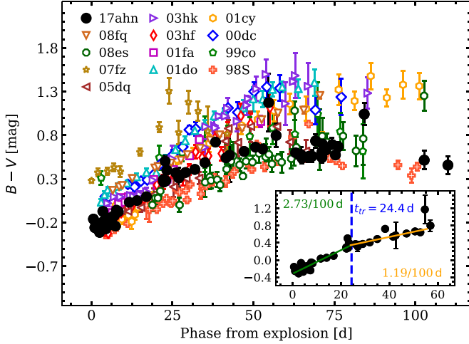
Figure 5. B - V color curve of SN 17ahn compared to the color evolution of the sample of Faran et al. (2014). The B - V color evolution of SN 1998S is also included for comparison. Magnitudes were corrected for the total (Galactic + host) extinction.
