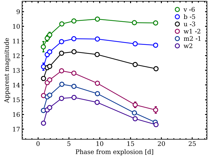
Figure 7. Swift UVOT light curves of SN 17ahn. Magnitudes were calibrated to the Vega photometric system and have not been corrected for extinction.
