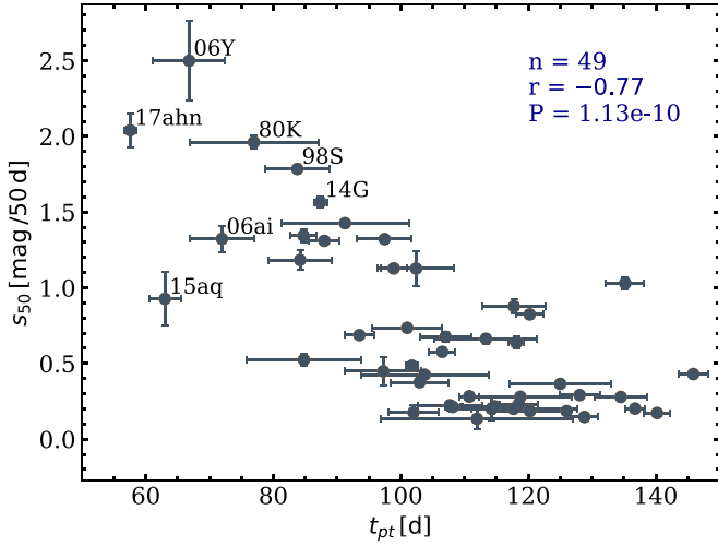
Figure 4. V-band decline rate measured at +50 days ( s_{50} ) vs. t_{pt} (see the main text) for the sample of Type II SNe of Valenti et al. (2016), including SN 17ahn and SN 1998S. n is the number of objects in the sample, r the Pearson s -correlation coefficient, and P is the probability of obtaining a correlation by chance.
