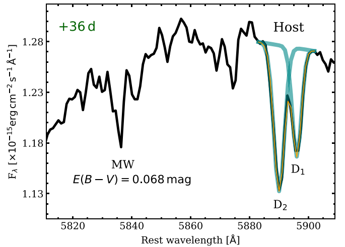
Figure 2. Zoom-in of the 5820–5900 Å region of the spectrum obtained on 2017 March 15 (36 days after explosion). Galactic DNa I and host absorption features are clearly visible. A multi-Gaussian fit (yellow line) of the marginally resolved host features including the single components (cyan lines). The spectrum is corrected for the recessional velocity of SN 2017ahn.
