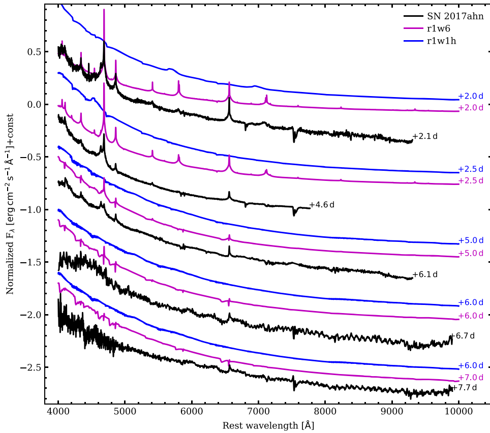
Figure 17. Comparison of the early ( t \lesssim 8 days) spectra of SN 2017ahn, corrected for the total reddening reported in Section 2, with a selection of Dessart et al. (2017) models. Model r1w1h reproduces the shape of the continuum at all phases well, although it does not show emission features observed in the early spectra of SN 2017ahn. Model r1w6 is able to reproduce both the spectral continuum and most of the emission lines at t > +2.5 days, while at +2 days the overall spectral features are not reproduced well by any of the models presented in Dessart et al. (2017). These models were chosen because their evolutions are similar to that of SN 2017ahn, including the high-ionization features (e.g., Ne III, He II, and IVC III) at early phases, the shape of the continuum, and the timescale at which the spectra evolve (e.g., all other models have a much faster evolution; high-ionization features disappear a few hours after the shock breakout; see Figures C.1–C.7 in Dessart et al. 2017). These correspond to a progenitor radius R_* = 501 R_\odot , with mass-loss rates 10^{-6} (r1w1h), and to 10^{-2} M_\odot \text{ yr}^{-1} (r1w6, with \dot{M} = 10^{-6} M_\odot \text{ yr}^{-1} beyond 5 \times 10^{14} cm, see the main text and Dessart et al. (2017) for more details).
