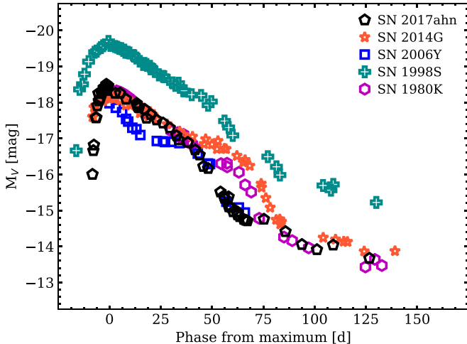
Figure 6. Absolute V-band light curve of SN 17ahn compared to those of other transients showing a similar photometric evolution (see the main text).
