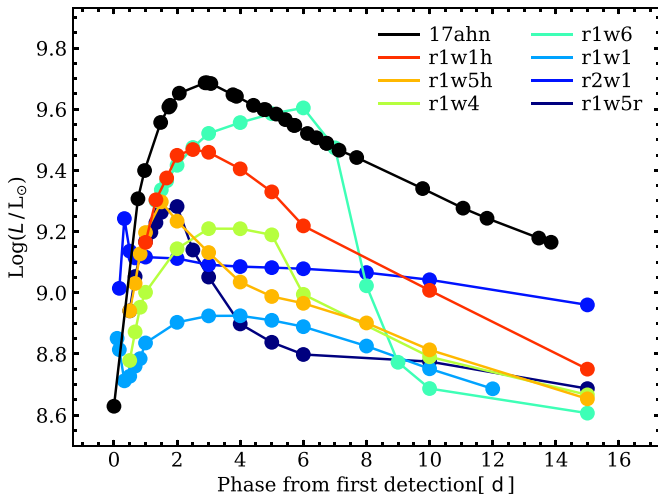
Figure 18. Comparison of the pseudo-bolometric light curve of SN 2017ahn with the uvior models of Dessart et al. (2017). Model r1w1h, corresponding to a progenitor radius R_* = 501 R_\odot with a mass-loss rate \dot{M} = 10^{-6} M_\odot \text{ yr}^{-1} and an atmospheric density scale height H_\rho = 0.1 R_* ( H_\rho = 0.3 R_* down to \rho = 10^{-12} \text{ g cm}^{-3} ; see the main text and Dessart et al. 2017 for details) reproduces the shape of the light curve well, although with a slightly fainter luminosity at all phases.
