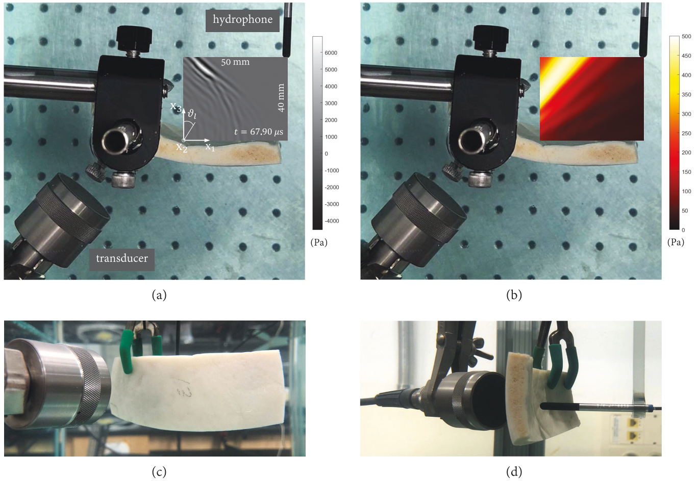
Fig. 9. Experimental setup for the parietal bone cut of Fig. 2(c). (a) Scan area and snapshot of the pressure field p(t, x_1, x_3) at 67.90 \mu s . (b) RMS plot of the pressure field. (c) and (d) Lateral views.
