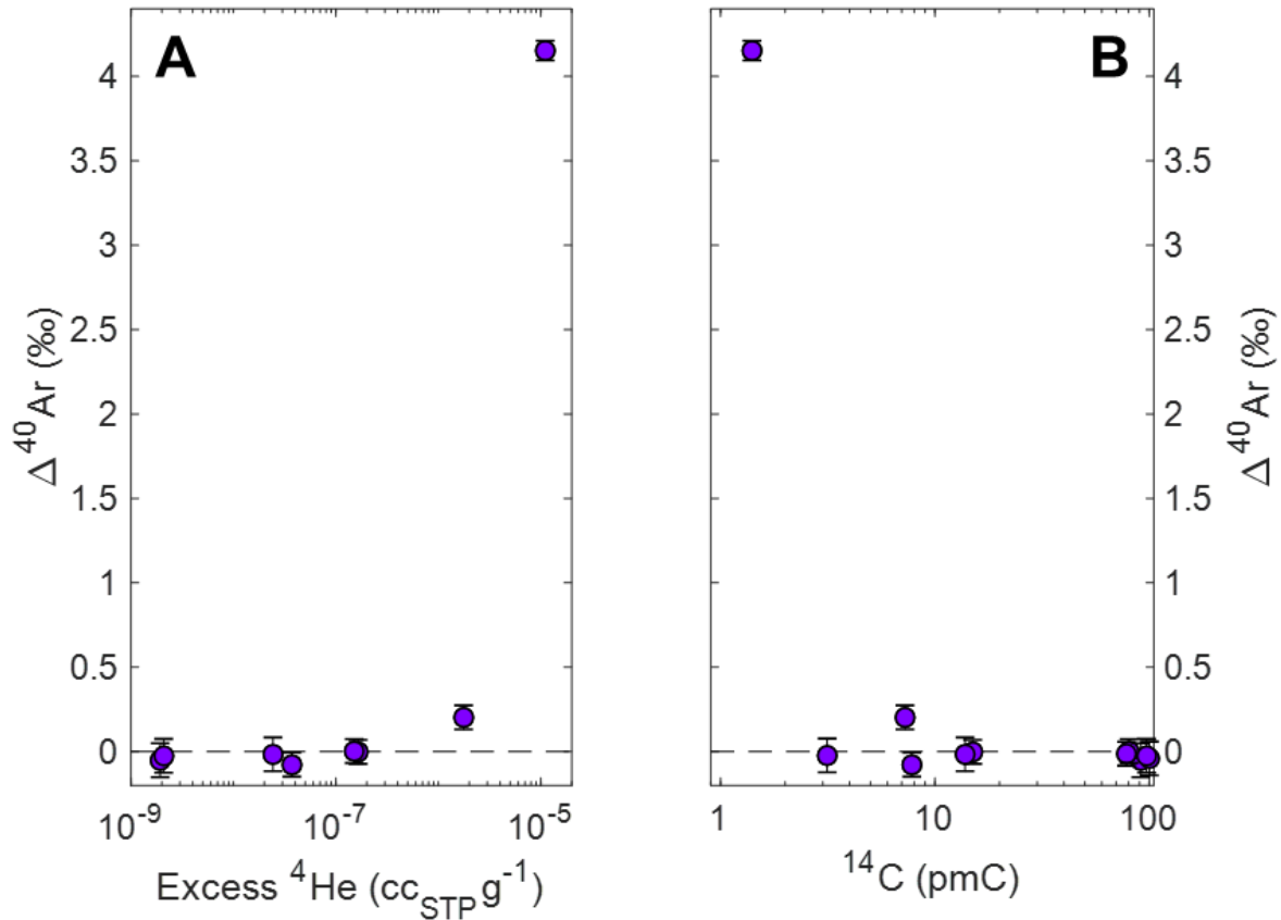
Figure 8: Mojave Desert replicate-mean \Delta^{40}\text{Ar} versus excess ^4\text{He} (panel A) and ^{14}\text{C} activity (panel B). Note that excess ^4\text{He} data are available for only 8 of 11 total Mojave Desert wells sampled for Ar isotope analysis, while ^{14}\text{C} data are available for all 11 wells. Error bars indicate \pm 2 SE.
