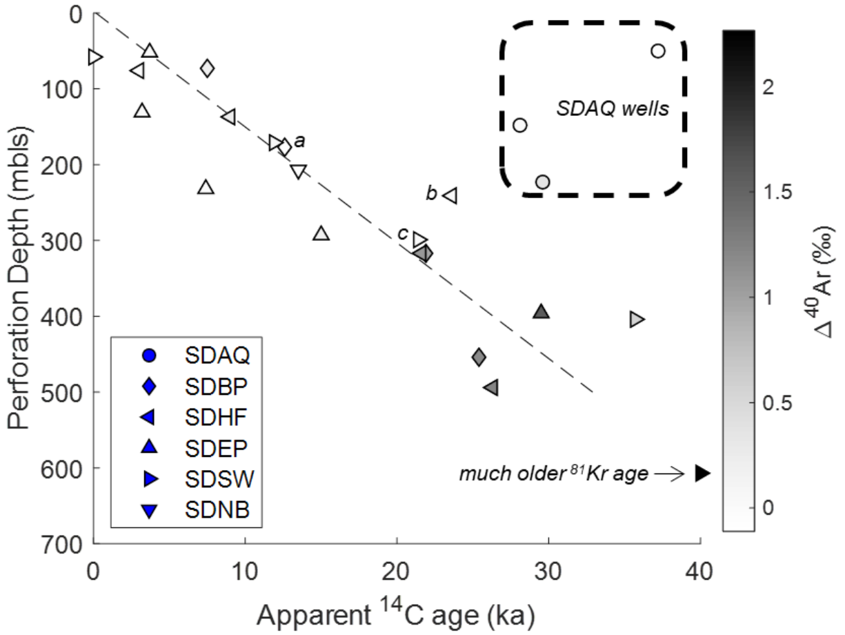
Supplementary Figure S3: Depth-age relationship for all San Diego groundwater wells included in this study. Excluding the shallow artesian SDAQ wells (n=3) and the deep SDSW well containing ^{14}\text{C} -free groundwater dated to be ~300 ka old by ^{81}\text{Kr} , the remaining wells (n=19) show a remarkably consistent linear trend ( R^2=0.80 ) with a slope of 0.066 \text{ ka m}^{-1} .
