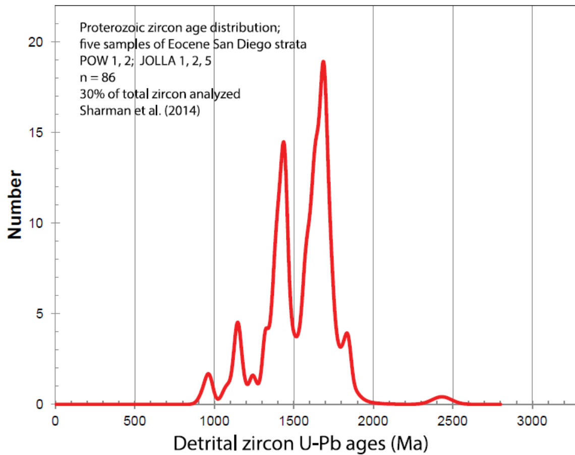
Supplementary Figure S4: Histogram of U-Pb ages (Ma) from n=86 zircons analyzed from five samples of Eocene strata in San Diego. Adapted from Sharman et al. (2014).
