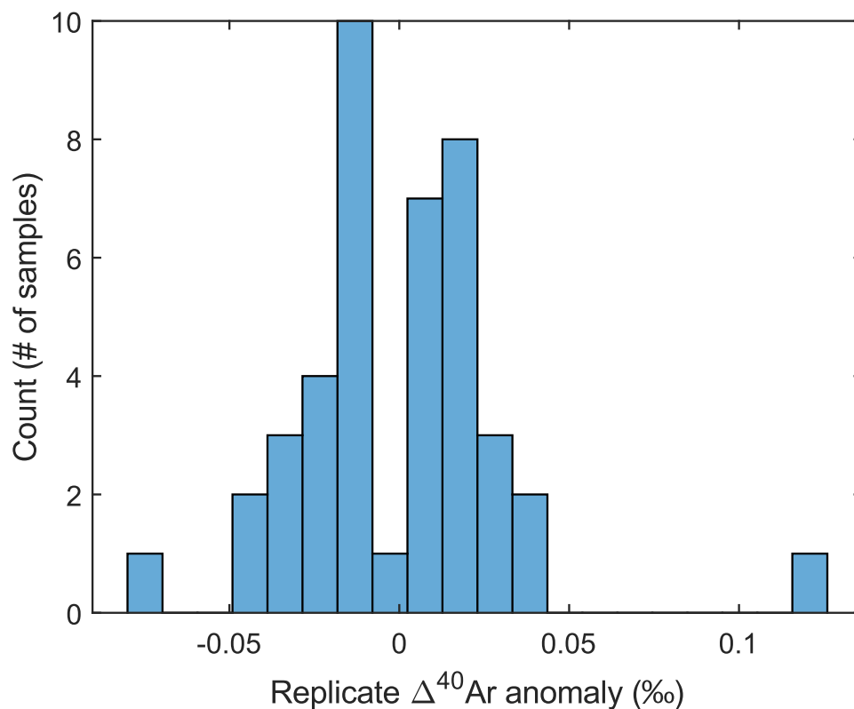
Supplementary Figure S2: Histogram of replicate anomalies in \Delta^{40}\text{Ar} from the replicate-mean value, across replicate 2-L groundwater samples from a given well. Of the 58 total measurements in this study (from 36 total wells), 42 samples were replicates from 20 wells. Conservatively, we adopt a 2- \sigma uncertainty of \pm 0.1\text{‰} for a single measurement, as described in section 2.
