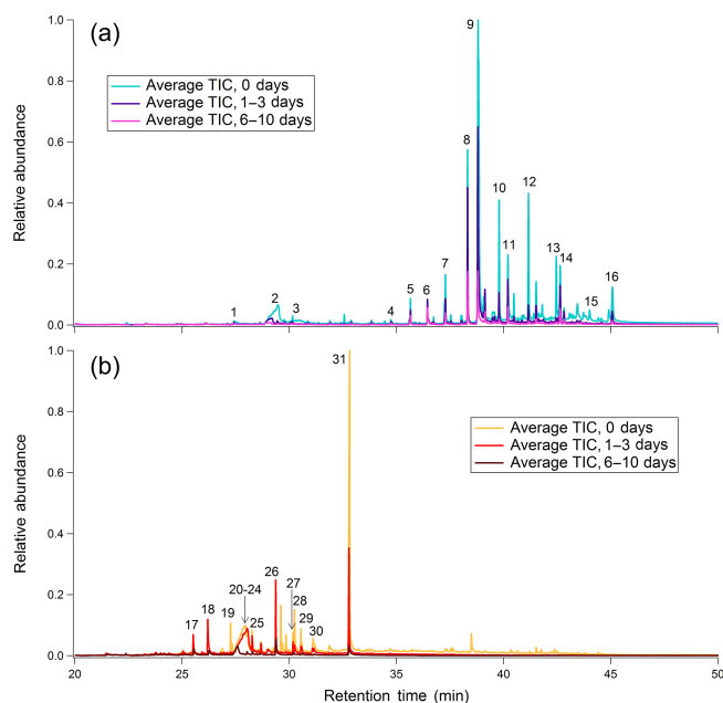
Figure 2. Chromatograms for (a) leaf BBOA and (b) heartwood BBOA at different levels of oxidation. Corresponding names and structures for numbered compounds are given in Table S5 and Fig. S9. For each plot, all traces are normalized to the point of highest abundance within the average unaged chromatogram.
