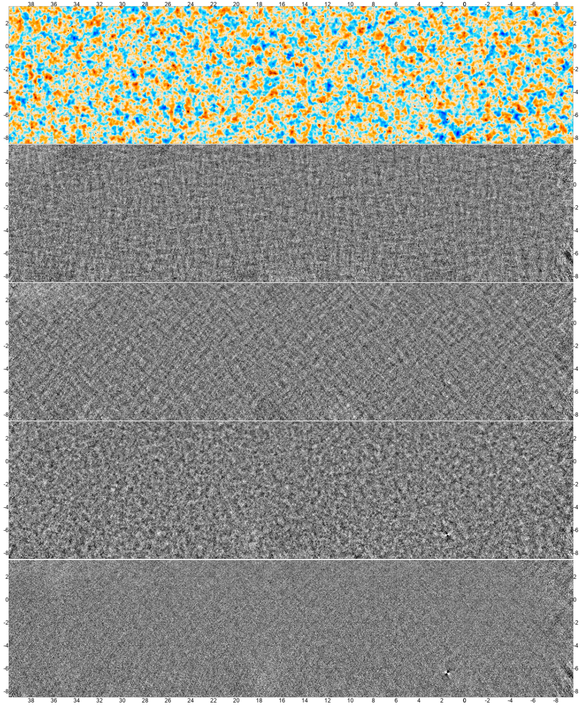
Figure 6. Rectangular cutout of the s13–s16 98 GHz maps in the D56 region. The selected area covers 630 \text{ deg}^2 of the sky. To visually highlight the wide range of measured angular scales, modes with |\ell| \lesssim 150 and |\ell_x| \lesssim 5 have been filtered out. The top panel shows temperature fluctuations in a range of \pm 250 \mu\text{K} . The remaining four black-and-white panels show (top to bottom) Q , U , E -mode, and B -mode polarization measurements in a range of \pm 30 \mu\text{K} . The x-axis (y-axis) shows the RA (Dec) coordinates in degree.
