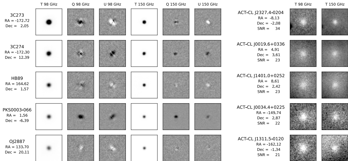
Figure 10. Sample of compact arcminute-scale objects detected in the ACT DR4 maps. All thumbnails are extracted by reprojecting a subset of the s13–s16 single-frequency map onto the plane tangent to the source coordinates to remove declination-dependent distortions. Each thumbnail has an extent of 15 \times 15 arcminutes and a resolution of 0.1 arcmin. (Left panel) Top-five highest signal-to-noise point sources detected in temperature at 150 GHz, ordered (top to bottom) by decreasing peak temperature. The colors (white to black) cover a range of [0, 5] \times 10^4 \mu\text{K} in temperature and \pm 1.5 \times 10^3 \mu\text{K} in polarization. No correction for the T-to-P leakage from the main-beam was applied. (Right panel) Top-five highest signal-to-noise SZ-selected galaxy clusters detected in a combination of the 98 and 150 GHz temperature maps, ordered (top to bottom) by decreasing signal-to-noise ratio. The colors (white to black) cover a range of [-500, 250] \mu\text{K} . An offset computed for each thumbnail (excluding the central source) is removed.
