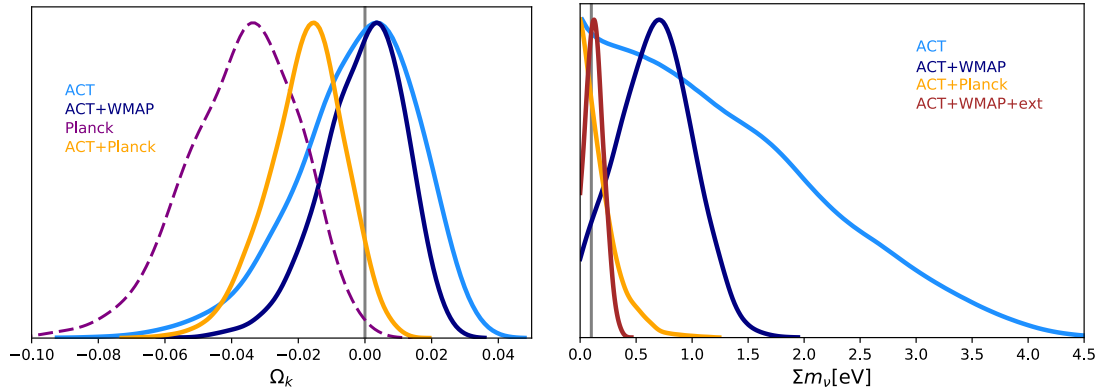
Figure 21. Constraints on the CMB-derived curvature parameter (left) and the sum of neutrino masses (right). These limits are driven by the lensing information in the power spectrum, as well as the primary CMB signal for neutrino mass. With the new ACT data we find no evidence of deviation from flatness, supporting the interpretation that the Planck primary CMB constraint (shown in purple for reference) is a statistical fluctuation. The neutrino mass is poorly constrained from ACT alone without the large-scale information. ACT+WMAP combined with external datasets (Planck lensing and BAO) gives \Sigma m_\nu < 0.27 eV at 95% confidence compared to < 0.19 eV at 95% confidence from Planck with the same data combination and same \tau prior. The standard model value for a flat Universe and the expected neutrino mass in an inverted hierarchy are shown with vertical grey lines.
