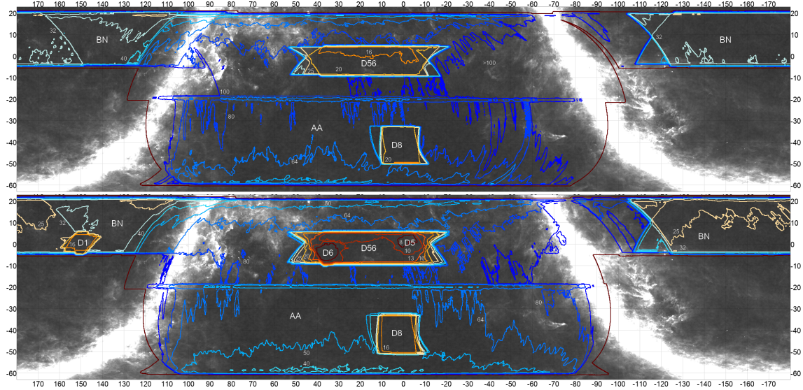
Figure 4. ACT DR4 survey depth and sky coverage maps for 98 GHz (top panel) and 150 GHz (bottom panel) in Equatorial coordinates. Lines at constant map-noise are plotted ranging from 7.5 \mu\text{K-arcmin} (red) to 101 \mu\text{K-arcmin} (blue). The Planck 353 GHz intensity map is shown in the background. The x-axis (y-axis) shows the RA (Dec) coordinates in degree.
