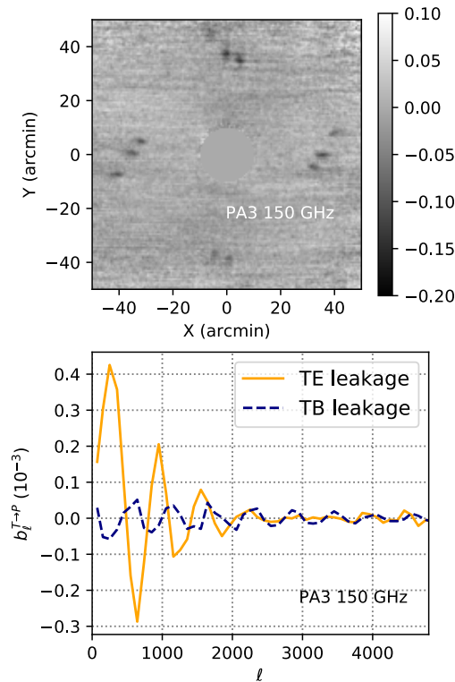
Figure 3. Weak polarized sidelobes in the PA3 150 GHz detectors. (Top panel) Map of the polarized sidelobes, obtained by stacking 20 observations of Saturn. The main lobe of the beam is at the origin and is masked in this image. The grayscale is linear in units of 1/1000 of the main beam peak, with positive (negative) numbers indicating polarization parallel (perpendicular) to the radial direction. The sidelobes consist of four groups of compact features, at 30 to 40 arcminutes from the main beam. (Bottom panel) The effect of unmitigated sidelobes on CMB spectrum measurements, expressed as transfer beam functions b_\ell^{T \rightarrow E} and b_\ell^{T \rightarrow B} . The sidelobes are strongly polarized in a direction perpendicular to the line connecting them to the main beam; this results in leakage that is primarily from temperature into E-mode polarization. Note that these sidelobes are projected out of the data prior to mapping the CMB, so the net leakage in the resulting spectra will be strongly suppressed relative to what is shown here.
