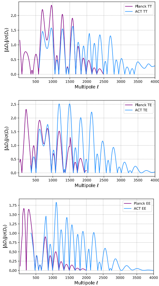
Figure 23. ACT and Planck signal-to-noise contributing to the estimate of the Hubble constant as function of multipole. The relative constraining power of each experiment is shown with the difference between two theoretical models with widely-spaced Hubble constants (63 and 76 km/s/Mpc, both consistent with the WMAP data to within 2\sigma ) normalized by the power spectrum error bar. This highlights the new information in the ACT DR4 data and their complementary with Planck: the largest contribution from ACT comes from the TE spectrum in the range 1000 < \ell < 2500 and the small scales in TT at \ell > 2000 and EE at \ell > 1000 provide additional information.
