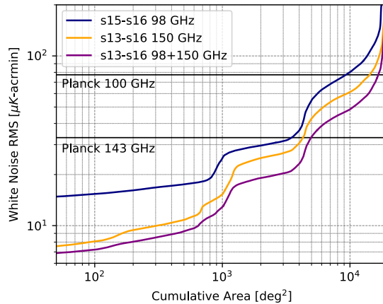
Figure 5. Map noise cumulative distribution function for 98 and 150 GHz and their combination. Two horizontal lines show the Planck full-sky averaged white-noise level for the 100 GHz and 143 GHz channels.
