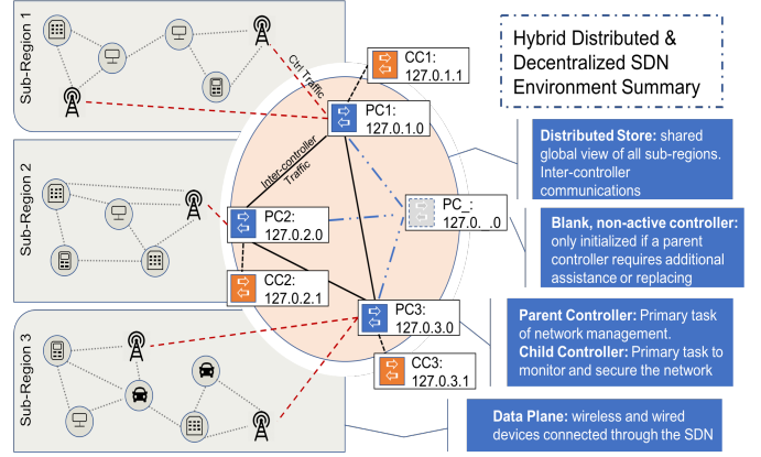
Fig. 1. Hybrid Distributed and Decentralized SDN Controller Architecture
