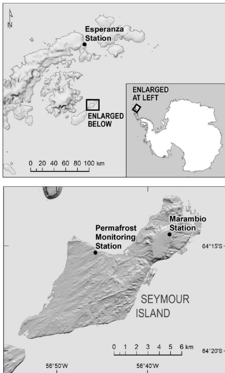
Figure 1. Locator image displaying Esperanza station (Argentina) situated in the Antarctic Peninsula region, and Seymour Island (with the permafrost monitoring station (Brazil) and Marambio station (Argentina) indicated. Topography (top map) from the National Snow & Ice Data Center at 1 km resolution (Liu et al., 2015). Topography (bottom map) from the
