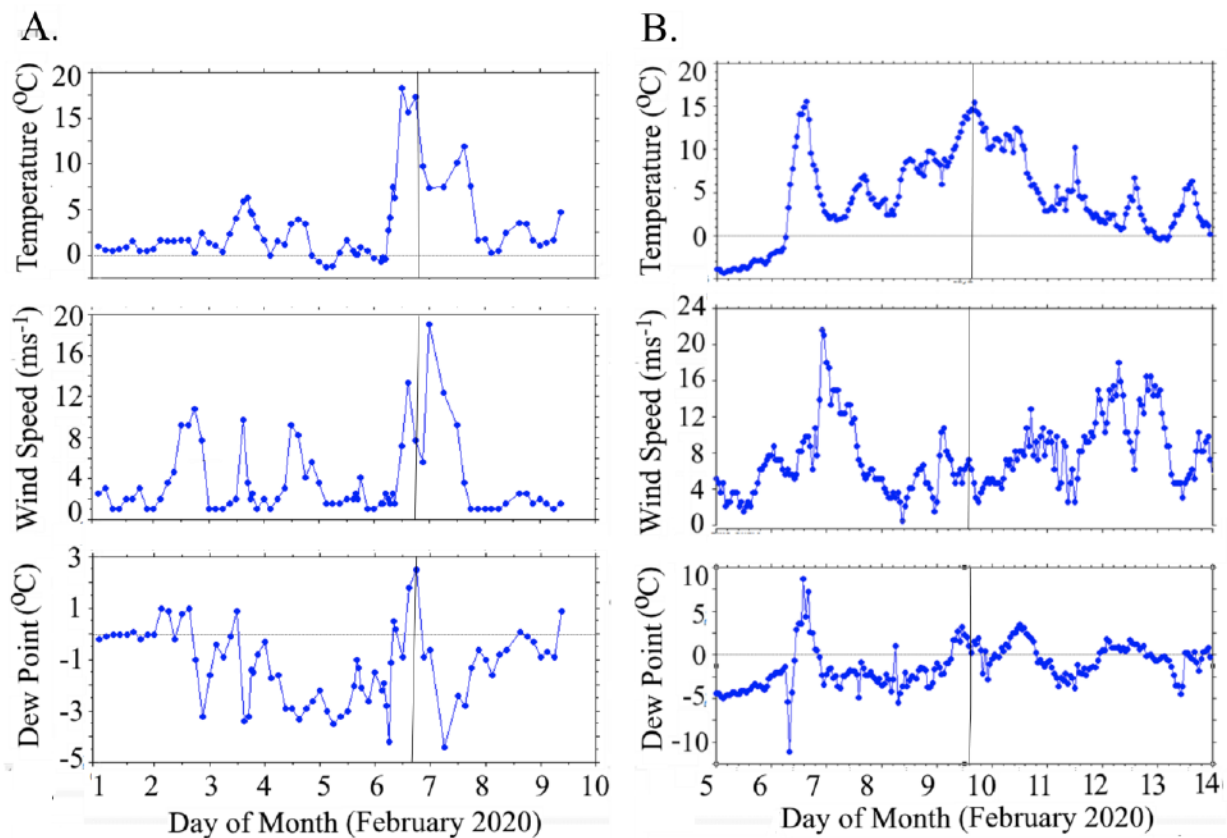
Figure 2. Meteorograms of Temperatures (top in ^{\circ}\text{C} ), Wind Speeds (middle in \text{ms}^{-1} ) and Dew Points (bottom in ^{\circ}\text{C} ) for A. Esperanza station (Argentina) and B. Marambio station (Argentina) on Seymour Island (located near the Brazilian permafrost monitoring station, see Figure 1) for selected days in February 2020. A and B are constructed so they are each centered about the specific days under investigation (6 Feb, Esperanza; 9 Feb, Seymour Island). The thin black lines at 15 UTC (1200 LST) 6 Feb 2020 (A) and 15 UTC (1200 LST) 9 Feb 2020 (B) indicate times of the specific observations under investigation.
