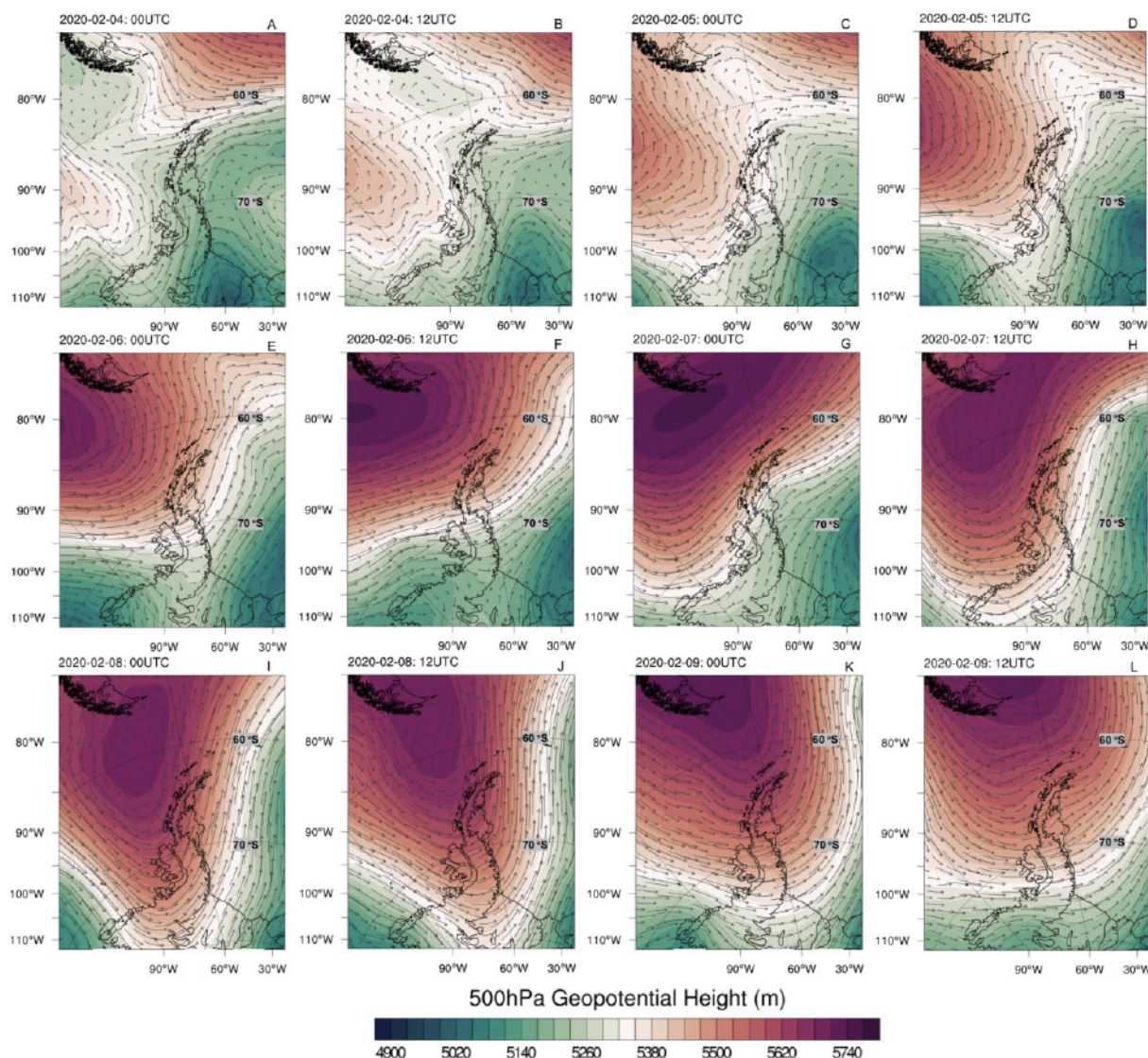
Figure 3. ERA5 reanalysis regional 500hPa heights (geopotential meters) together with 500 hPa vector winds for the Antarctic region for the period 2020-02-04 (00UTC, A) to 2020-02-09 (12 UTC, L). The Esperanza 18.3° C data point occurred at approximately 15UTC 6 Feb 2020. The Seymour Island permafrost monitoring site 20.8° C data point occurred at approximately 15 UTC 9 Feb 2020.
