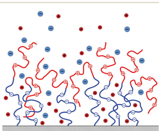
Fig. 1 Schematic representation of the end-tethered weak polyampholyte layer. The polymer layer consists of diblock polyelectrolytes end-grafted to a solid surface. The monomers, colored blue, are acidic in nature, meaning upon dissociation, they acquire a negative charge. The monomers, colored red, are basic in nature, being positively charged in their associated state. The monomers of acid-group carrying blocks and base-group carrying blocks are referred to as A and B monomers, respectively.
