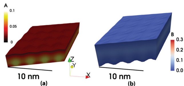
Fig. 11 Results of three dimensional calculations at pH = 3 for A_{20}B_{20} polymer at \beta\epsilon_{BB} = 6.0 . The corresponding grafting density is 0.1283 \text{ nm}^{-2} . The salt concentration is 0.01 M. Here, 50 percent of both A and B monomers are dissociable. The pattern was generated by plotting the iso-density surfaces with volume fraction 0.02 or more for both A and B. Both (a and b) were generated from the same camera view.
