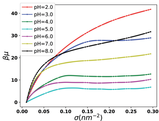
Fig. 9 Chemical potential of the polymer A_{20}B_{20} as a function of surface coverage at various pH values. The salt concentration is 0.01 \text{ M} . The above plots were generated for \beta\epsilon_{BB} = 6.0 . Here, 50 percent of both A and B monomers are dissociable.
