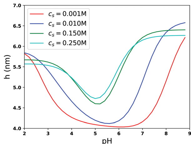
Fig. 7 The brush height as a function of pH at various salt concentrations. The grafting density corresponds to \sigma_p = 0.10 \text{ nm}^{-2} .
