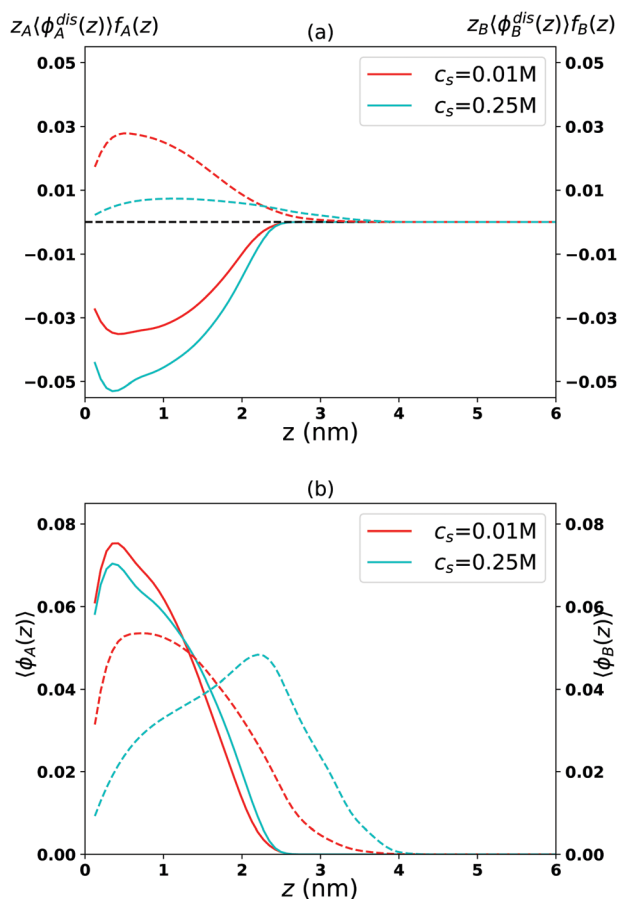
Fig. 5 The structural behavior of the polymer A_{20}B_{20} at pH 6. At this pH, an isolated A monomer would be mostly charged and a B monomer would be uncharged. The lower panel shows the volume fraction profiles of the A and B monomer of a A_{20}B_{20} brush. The solid and dashed lines correspond to the A and B monomers, respectively. The upper panel shows the charged monomer volume fraction profiles normalized by the valence of the monomer charge. z_A and z_B denote the valencies of dissociated A and B monomers, respectively. Two salt concentrations are considered. Namely c_s = 0.25 M and c_s = 0.01 M.
