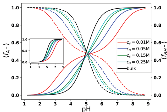
Fig. 2 The average degrees of charge fraction of A and B monomers in \text{A}_{20}\text{B}_{20} block copolymer as a function of pH for different bulk salt concentrations. All monomers of both blocks are dissociable. The grafting density, \sigma_{\text{p}} , is 0.10 \text{ nm}^{-2} . The solid lines and the dashed lines correspond to acidic and basic monomers, respectively.
