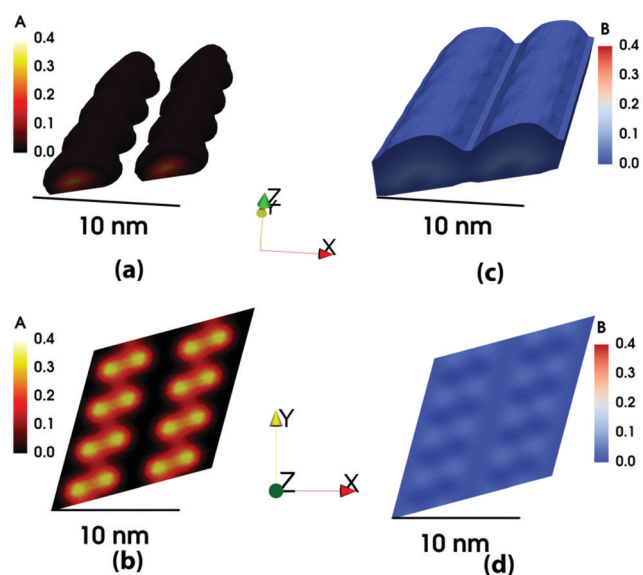
Fig. 12 Results of three dimensional calculations at pH = 3 for A_{20}B_{20} polymer at \beta\epsilon_{AA} = \beta\epsilon_{BB} = 6.0 . \beta\epsilon_{AB} = \frac{\beta}{2}\sqrt{\epsilon_{AA}\epsilon_{BB}} . The corresponding grafting density is 0.1283 \text{ nm}^{-2} . The salt concentration is 0.01 M. The fractions of dissociable monomers in both A and B blocks are 0.5. The scales in the figure are in nanometer. The top left panel shows the three dimensional view of the A monomers and the top right panel shows a similar view of the B monomers. The patterns were generated by plotting the iso-density surfaces with volume fraction 0.02 or more for both A and B. The bottom left panel shows the A monomer density map on a cross-sectional plane cut parallel to the grafting surface at z = 0.5 \text{ nm} . The bottom right panel shows the B monomer density map of the cut at z = 0.5 \text{ nm} .
