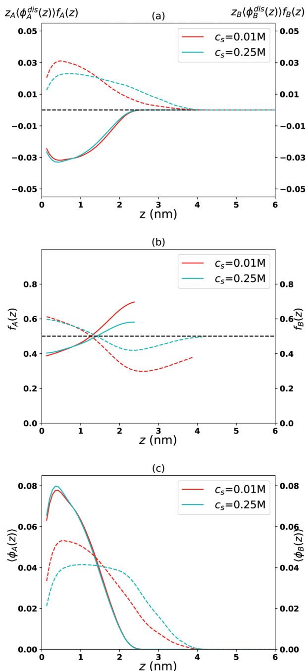
Fig. 6 The structural behavior of the polymer A_{20}B_{20} at pH 5. The fraction of charged acidic and basic monomers are shown in the middle panel. The solid and dashed curves represent A and B monomers, respectively. Note that although the dissociation profiles in the theory were computed for the whole region, only regions with non-zero monomer volume fraction ( >0.001 ) are shown. The corresponding monomer volume fraction profiles are shown in the lower panel. The top panel shows the charge profiles of A and B monomers. Salt condition identical to Fig. 4 and 6.
