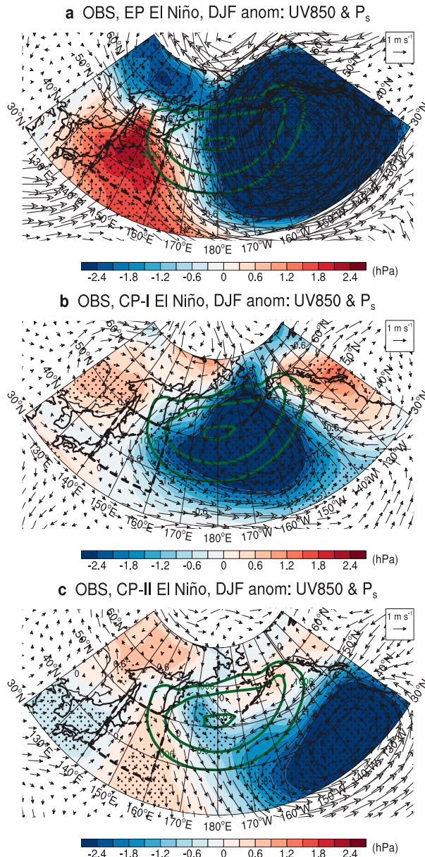
FIG. 6. Lambert conformal conic projection composite maps of anomalous low-level wind at the 850-hPa level (UV850; vectors; \text{m s}^{-1} ) and surface pressure ( P_s ; shading; hPa) during DJF for (a) EP, (b) CP-I, and (c) CP-II El Niños from the observations (OBS). Stippling indicates areas where the composite surface pressure anomalies are statistically significant at the 90% confidence level according to a Student's t test. The green contours over the central North Pacific indicate the climatological location of the Aleutian low, which is depicted by raw surface pressure levels from 998 to 1006 hPa (4-hPa intervals). The dashed areas are the selected region for the KAC in this study.
