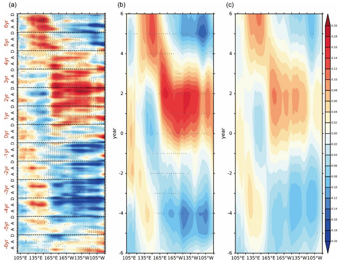
66 Figure S5. (a) Lagged regressions of monthly SSTA along the equator (5°S-5°N) Pacific, 67 unit in ^{\circ}\text{C}/100 \cdot \text{SSN} ) onto the yearly SSN during 1900-2018. (b) Same as (a) but 68 calculated with DJFMAM SSTA. (c) Same as (a) but calculated with the 7-year low- 69 pass filtered DJFMAM SSTA. Gray stipples indicate areas where the regressions are 70 statistically significance at the 95% confidence level determined using a Student's t- 71 test.
