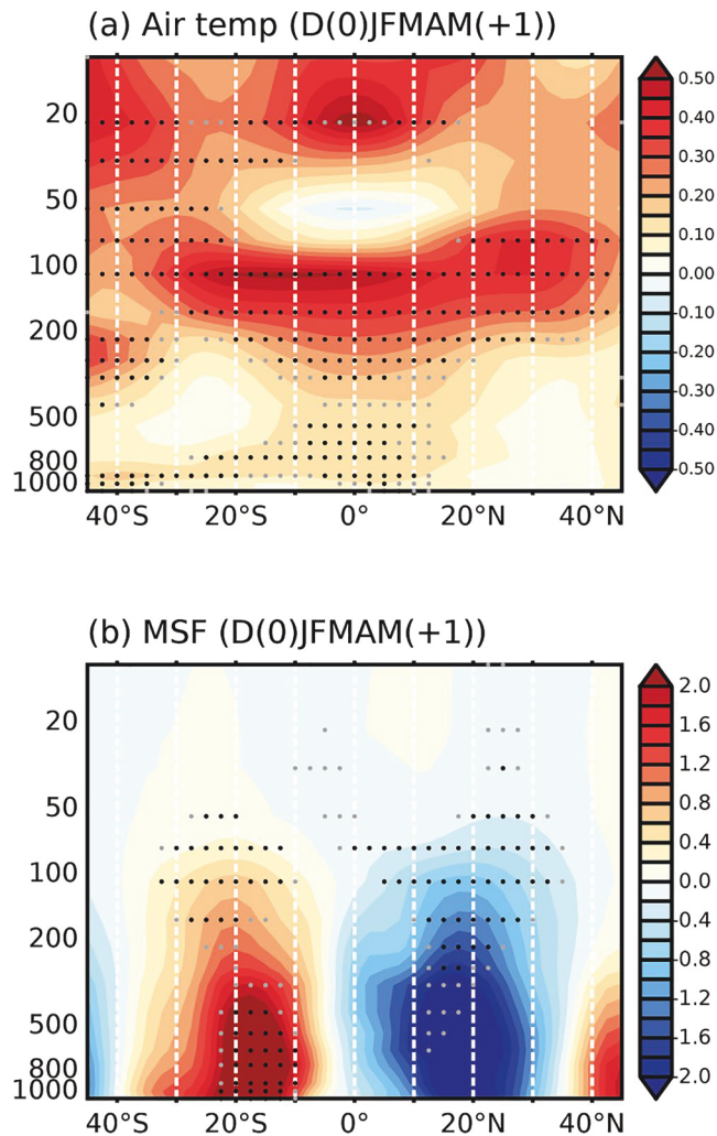
Figure 2. Regressions of DJFMAM zonal-mean global air temperature (a, ^{\circ}\text{C}/100 \times \text{SSN} ) and NEP (180°W–100°W) mass streamfunction profile (b, 10^{11} \text{ kg/s}/100 \times \text{SSN} ) onto the yearly SSN during 1948–2018. Positive (negative) values indicate clockwise circulations (counter-clockwise) in (b). Gray (black) stippled areas indicate significance at the 90% (95%) confidence level determined using a Student's t -test. DJFMAM, December to May; NEP, Northeastern Pacific, SSN, sunspot number.
