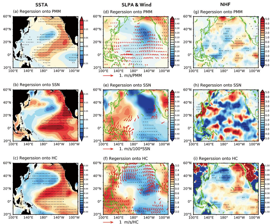
41 Figure S3. Regression of DJFMAM anomalies in SST ( ^{\circ}\text{C} ) with respect to the 42 DJFMAM PMM index (a), and yearly SSN (b), during 1948-2018. (c) Regression of 43 the 13-month running mean of SST anomalies onto the 13-month running mean of the 44 NE Pacific HC index (multiplied by -1). (d-f) same as (a-c), but for anomalies in SLP 45 (hPa) and 1000 hPa wind. (g-i) same as (a-c), but for anomalies in net heat flux ( \text{W}/\text{m}^2 ). 46 In (d-f), only vectors at the 95% confidence level or higher are shown. Stippled areas 47 in each figure indicate significance at the 95% confidence level determined using a 48 Student's t-test.
