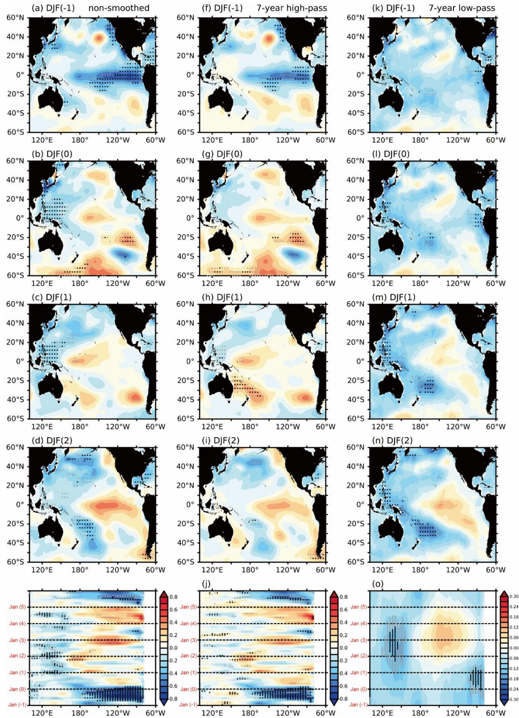
Figure S4. SSTA (unit in °C) composited from the 12 first-peak years of the solar cycle (1883, 1893, 1905, 1917, 1928, 1937, 1947, 1957, 1968, 1979, 1989, 2000; following Meehl and Arblaster, 2009) during (a) the DJF before the peak year (DJF -1), (b) the DJF of the peak year (DJF 0), (c) the 1 st DJF after the peak year (DJF 1), (d) the 2 nd DJF after the peak year (DJF 2). (e) Evolution of the composite monthly SSTA along the equatorial (5°S-5°N) Pacific from one year before to five years after the first-peak year and calculated with the original SST anomalies. (f-j) same as (a-e) but calculated using the 7-year high-pass filtered SSTA. (k-o) same as (a-e) but calculated using the 7-year low-pass filtered SSTA. The Least Squares Lanczos filter was used for the filtering. Gray (black) stipples indicate areas where the composites are statistically
