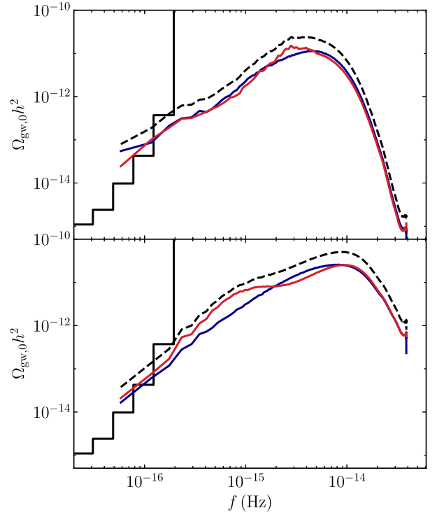
FIG. 3. Polarization components of the present-day gravitational-wave spectrum emitted by recombination (i.e., evaluated at z \approx 1100 ) for \alpha = 50 (top) and 70 (bottom). The plus and minus polarizations are in blue and red, respectively, while the total signal is portrayed in dashed black. Both panels fix m_\phi = 10^{-26} eV, f = 1.5 \times 10^{17} GeV, and \theta = 2 . In solid black is the upper bound as constrained by the CMB, computed in Ref. [54].
