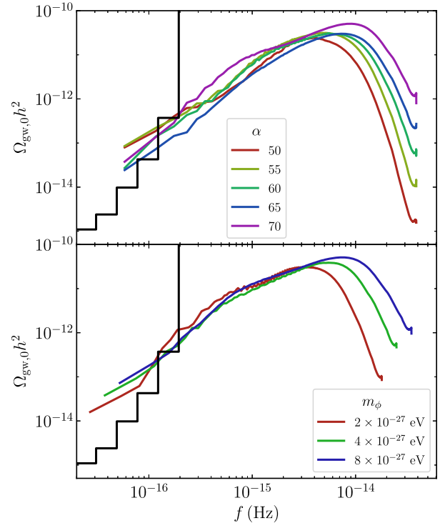
FIG. 2. Present-day gravitational-wave spectrum emitted by recombination (i.e., evaluated at z \approx 1100 ), fixing m_\phi = 10^{-26} eV and varying \alpha (top), and fixing \alpha = 70 and varying m_\phi (bottom). All simulations set f = 1.5 \times 10^{17} GeV and \theta = 2 . In black is the upper bound as constrained by the CMB, computed in Ref. [54].
