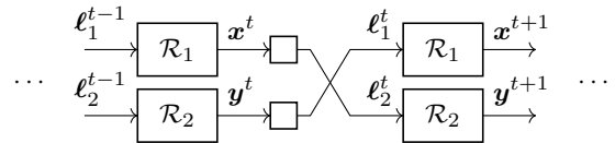
Figure 1. Self-play method for computing NE in EFGs.
