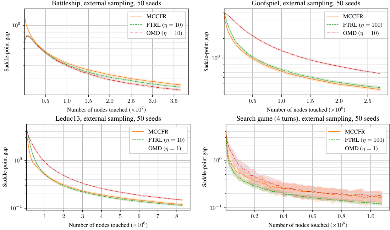
Figure 3. Performance of MCCFR, FTRL, and OMD when using the external sampling gradient estimator.
