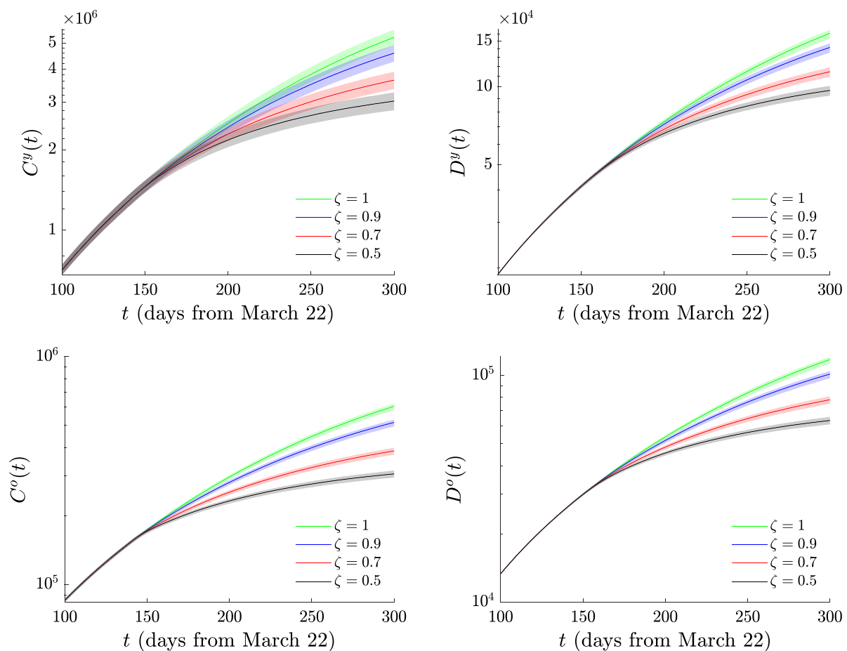
Fig. 9. Same as Fig. 5, but for the two-population model when additional measures are applied to the older (than 65) population, i.e. \zeta^o = 1 and \zeta^y \equiv \zeta . Notice the significant deviation of both the number of infections (left) and of the number of deaths (right), both for the younger (than 65) and the older (than 65) populations between current policy ( \zeta = 1 ) and the suggested additional intervention measures (by a factor of 0.5 to 0.9).
