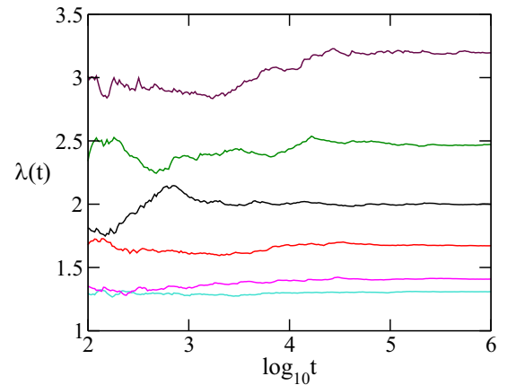
FIG. 11. The finite-time mLCE \lambda(t) for different \mu values ( \mu = 0.05, 0.1, 0.2, 0.3, 0.4, 0.5 , from bottom to top) and for the parameters ( a = 1.5 , h = 3 ). The value of \lambda(t) at t = 10^6 is shown in Fig. 10.
