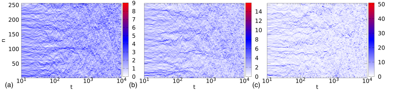
FIG. 3. The amplitude profiles in space ( n )-time ( t ) in the Gibbs regime for three different \mu values (a) \mu = 0.05 , (b) \mu = 0.2 , and (c) \mu = 0.5 at ( a = 1.5 , h = 3 ) for the system size N = 256 .
