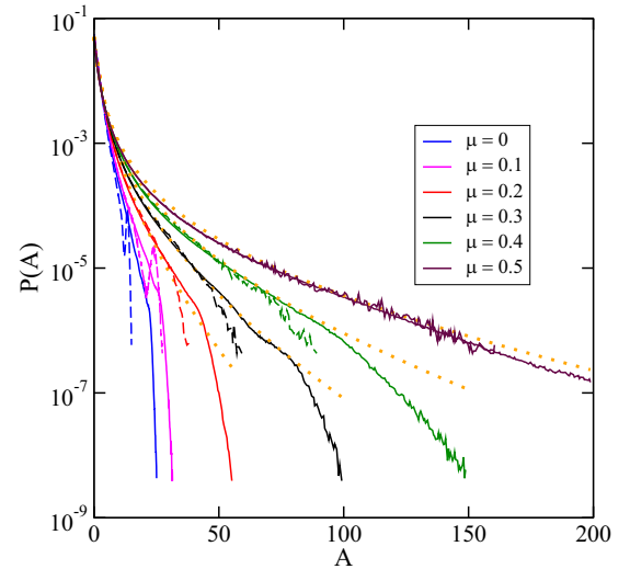
FIG. 5. The PDF of local norms (amplitudes) A_n = |\psi_n|^2 for different values of \mu for the parameter set ( a = 1.5 , h = 5 ). This arrangement is in the Gibbs regime for \mu > 0.17 and otherwise in the non-Gibbs regime. Different curves are associated with \mu = 0, 0.1, 0.2, 0.3, 0.4, 0.5 as shown in the legend. Dotted orange curves represent the results obtained analytically by the TIO method, while dashed and solid lines show the numerically generated P(A) at two different times T = 10^5 and T = 10^7 , respectively. TIO curves fit the numerical ones in the Gibbs regime, except for the large-amplitude tail region.
