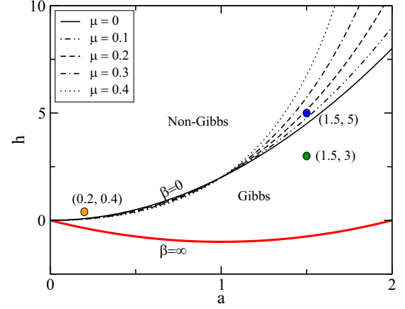
FIG. 1. The norm and energy density parameter space (a, h) of the SM. The area between the curves \beta = 0 (black thin lines) and \beta \rightarrow \infty (red solid thick line) in the parameter space (a, h) denotes the Gibbs regime of anticipated thermalization [Eq. (7) is valid] for a few values of the parameter \mu ( = 0, 0.1, 0.2, 0.3, 0.4 ) respectively represented by solid, dot-dot-dashed, dashed, dot-dashed, and dotted black curves. The area above \beta = 0 will be referred to as non-Gibbs, where Eq. (7) is invalid. The region below \beta \rightarrow \infty is forbidden for any microcanonical states. The green, blue, and orange symbols respectively represent (a = 1.5, h = 3) , (a = 1.5, h = 5) , and (a = 0.2, h = 0.4) .
