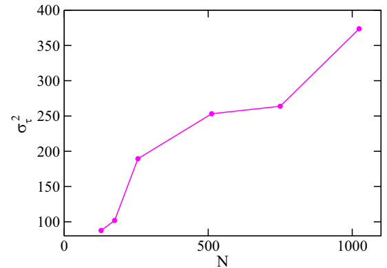
FIG. 8. The variance \sigma_\tau^2 for \mu = 0.05 and (a = 1.5, h = 5) as a function of system size N . This case corresponds to the non-Gibbs regime. The total integration time T = 10^7 . The results are averaged over 5 different initial conditions.
