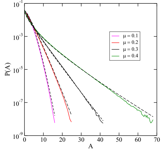
FIG. 2. The PDF of local norms (amplitudes) A_n = |\psi_n|^2 for different values of \mu for the parameter set ( a = 1.5 , h = 3 ). Dashed curves represent the results obtained analytically by the TIO method, while solid curves show the numerically generated PDFs. The total integration time is T = 10^7 . TIO curves nicely fit to numerical ones in the Gibbs regime.
