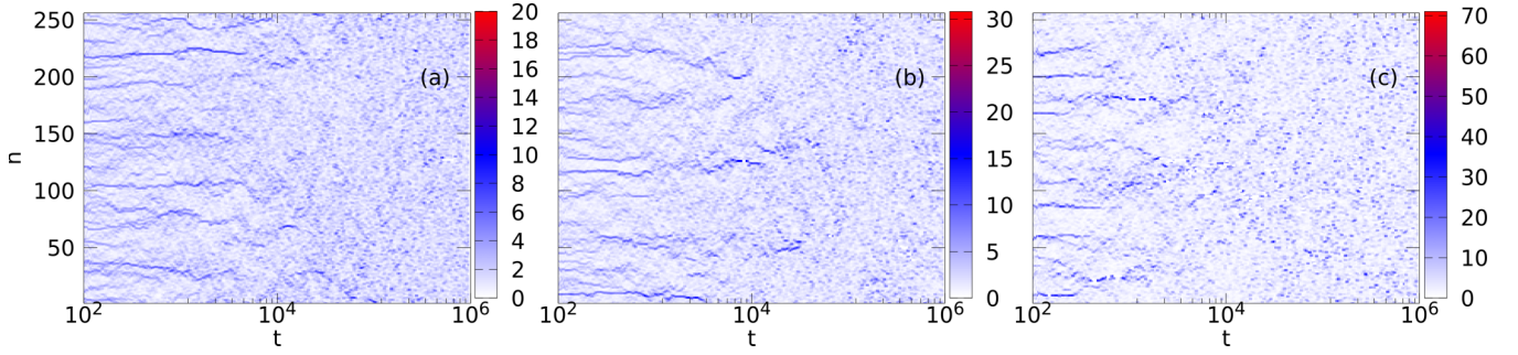
FIG. 6. In panels (a), (b), and (c), the amplitude profiles are respectively shown in the non-Gibbs regime ( \mu = 0.05 ), near the critical point ( \mu = 0.2 ), and in the Gibbs regime ( \mu = 0.5 ) for a = 1.5 , h = 5 , and N = 256 . In the non-Gibbs phase [panel (a)], the appearance of localized breathing structures is significantly more prominent than in the Gibbs regime [panel (c)].
