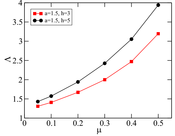
FIG. 10. The mLCE ( \Lambda ) for ( a = 1.5 , h = 3 ) (red squares) and ( a = 1.5 , h = 5 ) (black filled circles) as a function of \mu for N = 256 . In both cases the value of \Lambda increases with \mu . See Fig. 11 for the finite time mLCE \lambda(t) .
