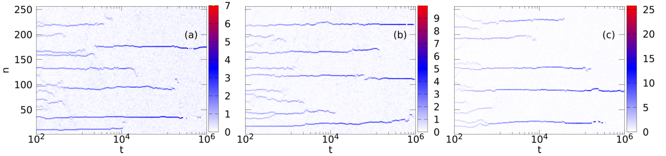
FIG. 9. The amplitude profiles in the non-Gibbs regime for (a) \mu = 0.05 , (b) \mu = 0.2 , and (c) \mu = 0.5 at a = 0.2 , h = 0.4 for N = 256 .
