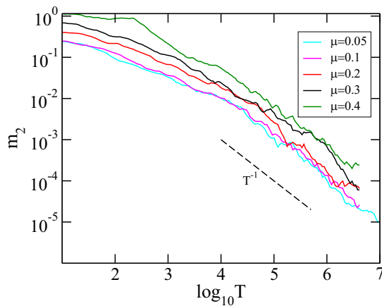
FIG. 4. The evolution of the second moment [ m_2(T) ] of FTA distributions of the integral local norms for the different values of \mu corresponds to ( a = 1.5 , h = 3 ). The dashed line represents m_2 \propto T^{-1} .
