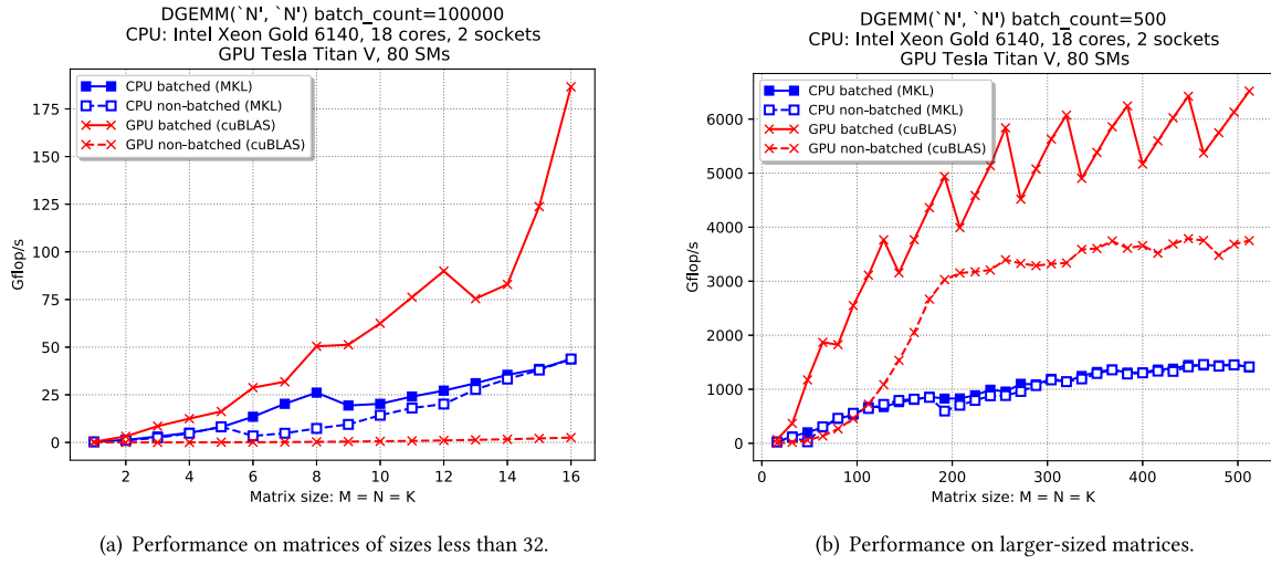
Fig. 3. Performance of batch DGEMM on Titan V GPU and dual 18-core Intel Xeon Gold 6140 (Cascade Lake) 2.30 GHz CPU in NVIDIA cuBLAS and Intel MKL.
