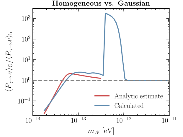
FIG. 3. An analytic estimate for the ratio of the probability of conversion with the Gaussian PDF vs that of the homogeneous assumption (red) for conversions that happen at z < 6 , with agreement between the two approaches corresponding to a conversion probability ratio of one (gray). The full numerical result is shown for comparison (blue). There are no conversions in the homogeneous limit for m_{A'} \lesssim 2 \times 10^{-14} eV [38].
