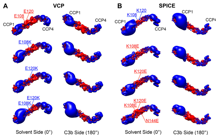
FIGURE 4 | Electrostatic potential maps for the (A) Vaccinia virus complement control protein (VCP) and (B) smallpox inhibitor of complement enzymes (SPICE), upon point mutations of the E108K, E120K, and E108K/E120K residues in VCP, and upon the reverse mutations of K108E, K120E, and K108E/K120E/N144E in SPICE. The electrostatic potential is represented as isopotential contour maps, with blue and red contours having isovalues of +2 and -2 k_B T/e^- , respectively. Two orientations of the ligands are shown, displaying their solvent side and the side binding C3b (upon a 180° rotation around the horizontal axis). The electrostatic potential calculations were performed with 150 mM ionic strength.
