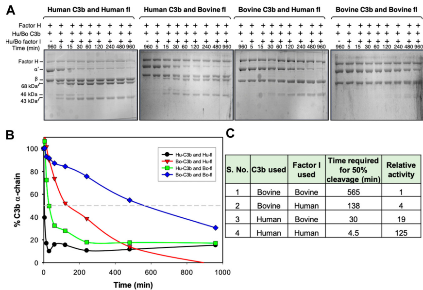
FIGURE 3 | Cofactor activity of human factor H for human and bovine C3b. (A) Analysis of cofactor activity by SDS-PAGE gel analysis. C3b (human or bovine) was mixed with human factor H and factor I (human or bovine), incubated at 37 °C for the indicated time, and examined for C3b cleavage ( \alpha' -chain cleavage) by running the reaction mix on SDS-PAGE. (B) The amount of \alpha' -chain at different time points was quantitated densitometrically and plotted against time. (C) Relative cofactor activity of factor H against human and bovine C3b in the presence of human or bovine factor I. The molar concentration of the complement components used in the cofactor assay was: 758 nM Hu/Bo C3b, 11 nM Hu/Bo factor I and 473 nM Hu factor H.
