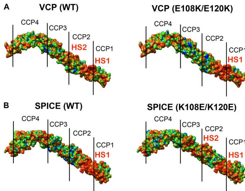
FIGURE 5 | Electrostatic Similarity Index (ESI), projected on the 3D structure of (A) the vaccinia virus complement control protein (VCP) and of (B) the smallpox inhibitor of complement enzymes (SPICE). ESI is computed and projected on the proteins as wild-type (WT, left panel) and upon mutation of the residues 108 and 120 (right panel). Observed electrostatic hotspots on the ligands are marked as HS1–HS2. The color scheme blue–green–orange represents low–to–high similarity, corresponding to ESI values of 0.4–0.7–1.0.
