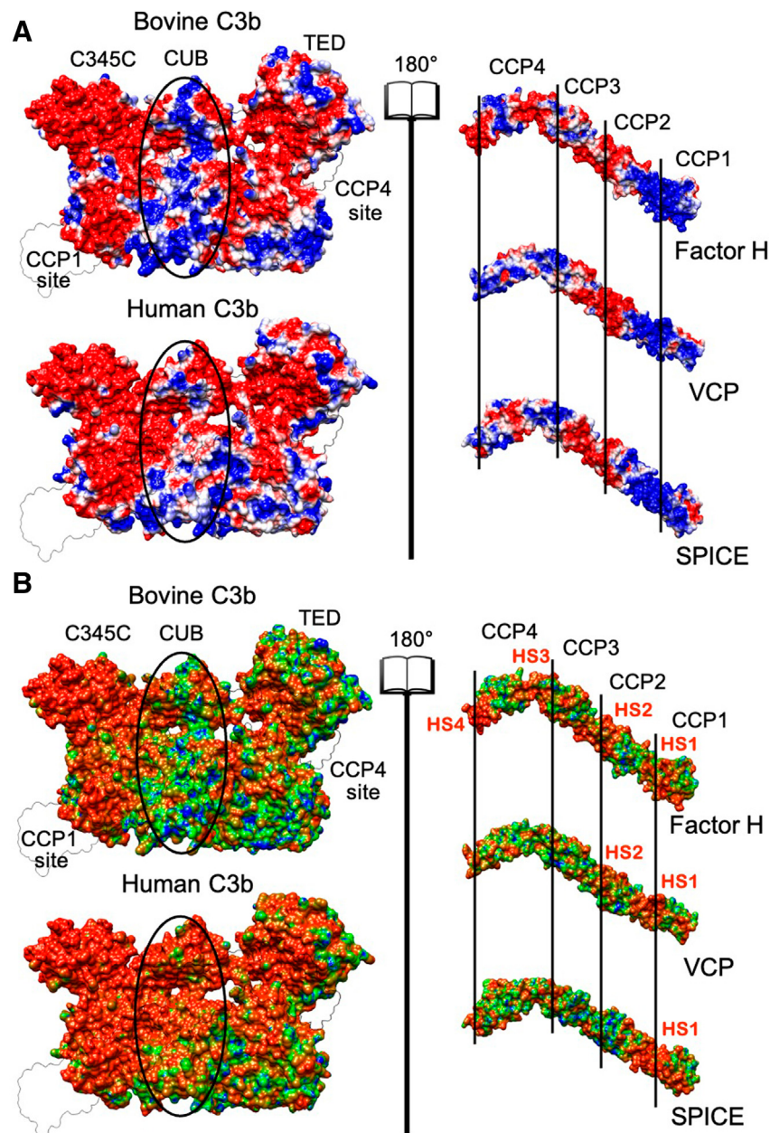
FIGURE 2 | (A) Electrostatic potential surface projection for the bovine and human C3b proteins (left panel) and for the Factor H, VCP and SPICE ligands (right panel). The left and right panels are separated by an “open book” view, which reveals the surfaces of contact at the interface of the protein-ligand complex. The protein domains of C3b (C345C, CUB, and TED) and the complement control protein (CCP) modules of Factor H, VCP and SPICE (CCP1–4) are also shown. On the 3D structure of C3b, the location of the CCP1 and CCP4 binding sites is also shown. The ellipses depict differences in the central regions of bovine and human C3b. The electrostatic potential is colored from red (negative) to blue (positive). (B) Electrostatic Similarity Index (ESI), projected on the 3D structure of the bovine and human C3b protein (left panel) and of the Factor H, VCP and SPICE ligands (right panel). Observed electrostatic hotspots on the ligands are marked as HS1–HS4. The color scheme blue–green–orange represents low–to–high similarity, corresponding to ESI values of 0.6–0.8–1.0 for the bovine and human C3b, and ESI values of 0.4–0.7–1.0 for the ligands.
