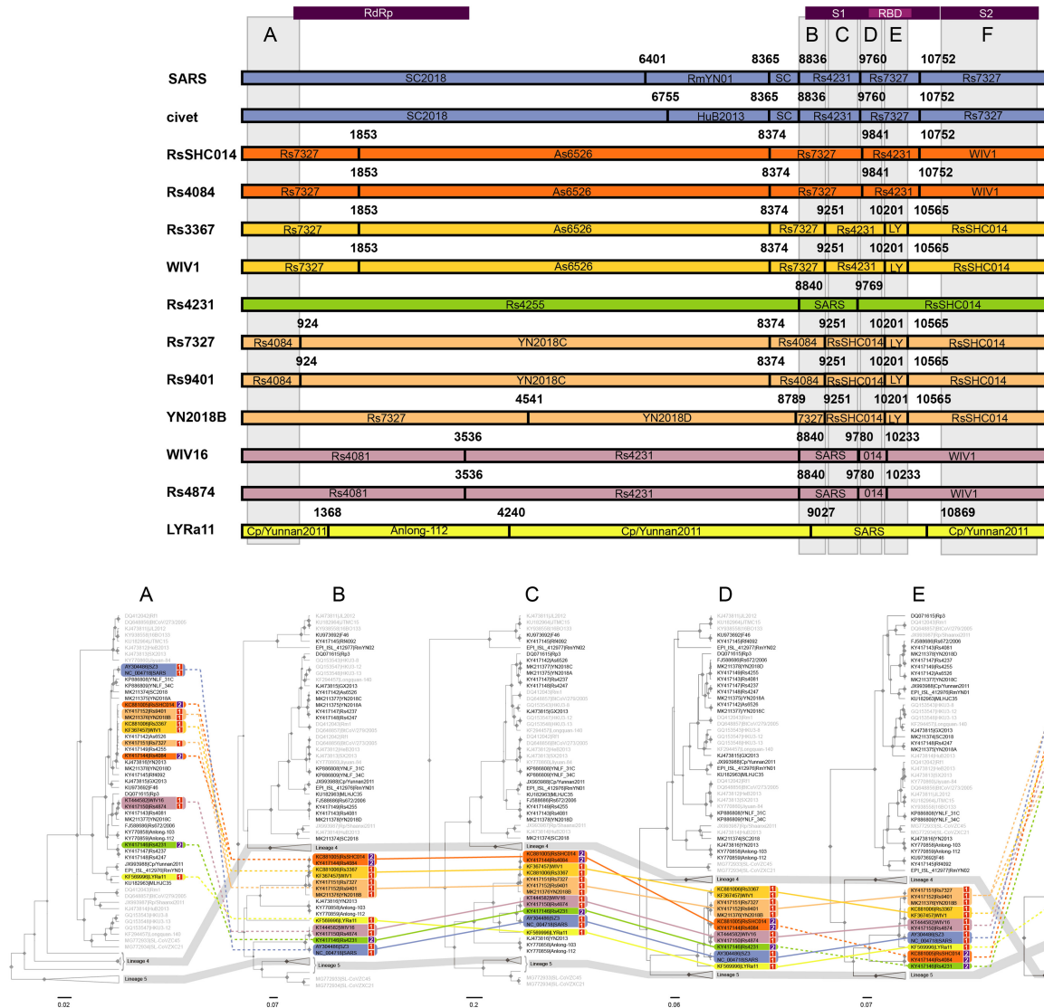
Figure 6. Recombination breakpoints detected in Lineage 1 ACE2-using sequences. The top of this figure illustrates that the recombination suggested by the change in topology in Fig. 2 for 13 Lineage 1 viruses is supported by formal breakpoint analysis. The breakpoints detected for each of the 13 recombinant Lineage 1 sequences with ACE2-using structure (no deletions) are shown. Sequences that are nearly identical are colored the same for simplicity. The bars represent the sequence of genome beginning 750 bp before RdRp spanning through the end of S2 (SARS-CoV-2 nucleotides 12,681 through 25,176) and each box within represents a recombinant section within the sequence. The breakpoints correspond to those identified in Table 2 . Numbering is relative to the alignment. The parental sequence is shown within each box. Sequences identified as the minor parent by 3SEQ were labeled within the breakpoint margins and the major parent outside. Six regions where these sequences appear to be free of recombination are labeled A–F and a corresponding phylogeny for each region is shown below. Regions A and E were further tested for recombination breakpoints in all sequences, not just the 13 Lineage 1 viruses, and were found to be breakpoint-free. The topology of regions A and E is not different enough from Fig. 2 to suggest that recombination within RdRp or RBD significantly changed the interpretation of our results. For each region, sequences were tracked with connecting lines of corresponding color to identify where recombination may have occurred between Lineage 1 and Lineage 5 and hypothesized events are specifically marked with dotted lines. This highlights the secondary recombination of Rs4084 and RsSHC014 in region E on top of the primary recombination in regions B through E. Sequence names of Lineage 2 and 3 viruses are greyed out and Lineages 4 and 5 are collapsed and highlighted in darker grey to make the changes in topology between the trees more visible.
