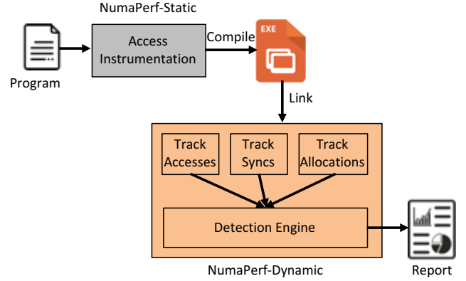
Figure 2. Overview of NumaPerf
