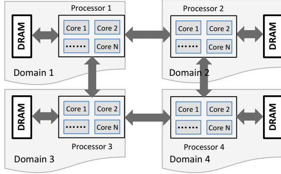
Figure 1. A NUMA architecture with four nodes/domains
