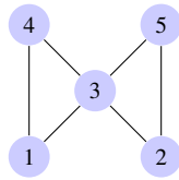
Fig. 6.1 The set T = \{1, 2, 3\} neither contains nor is contained in a clique.
