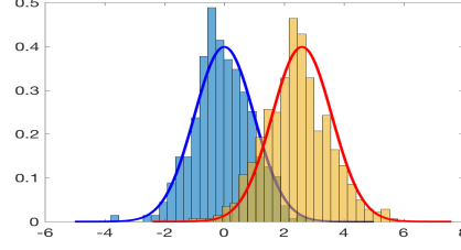
Figure 2. Histograms of \sqrt{(B_{n,4}/8)} \cdot \hat{C}_4^{-1/2} \hat{\chi}_{gc}^{(4)} for the null hypothesis (light blue) and the alternative hypothesis (yellow). The blue and red curves are densities of N(0, 1) and N(\delta_{gc}^{(4)}, 1) , respectively, which support our results on asymptotical normality.
