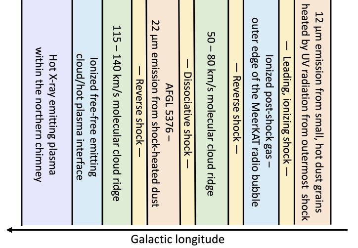
Fig. 8. Schematic representation of the structure of the northwestern edge of the chimney.
