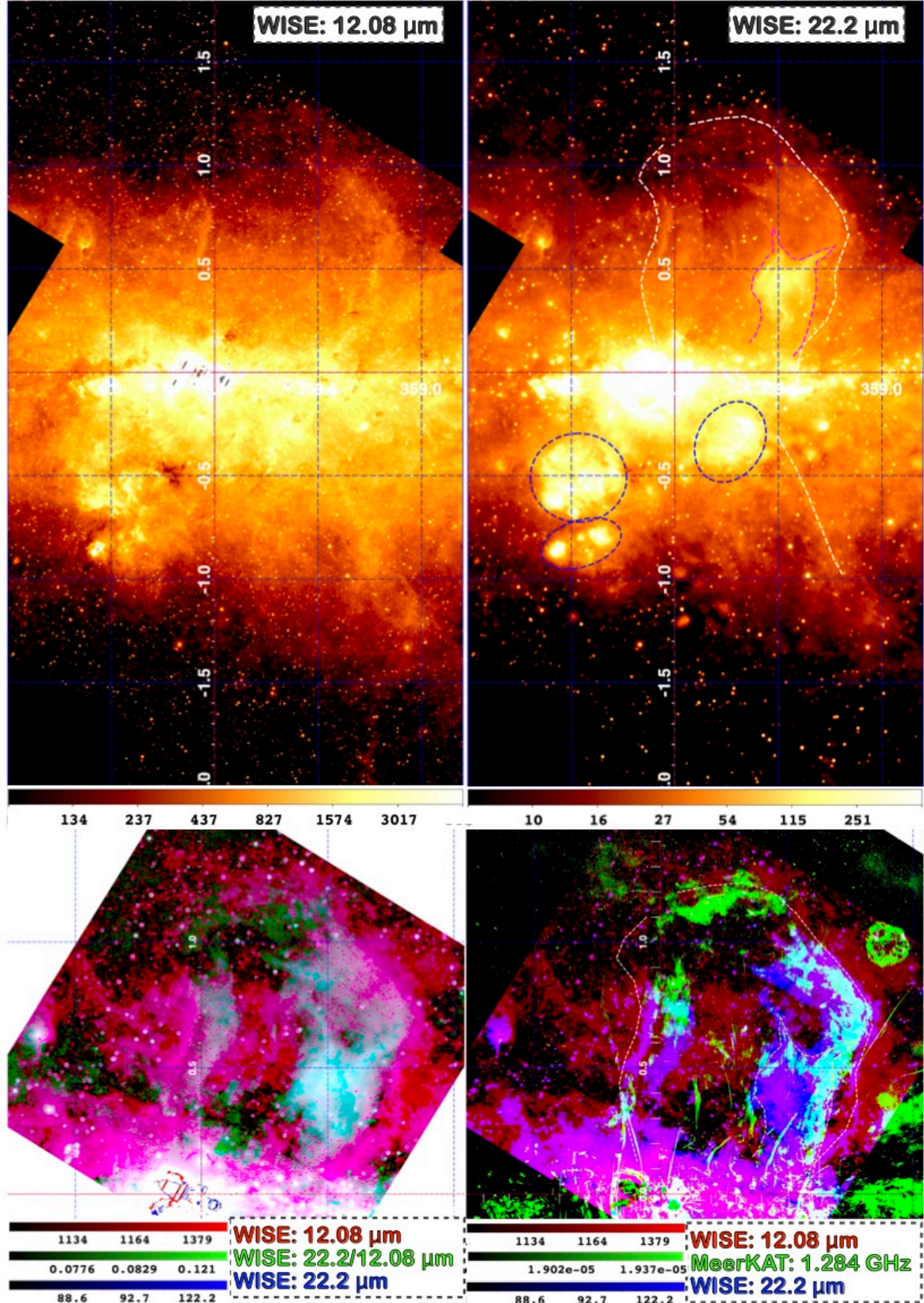
Fig. 6. Mid-IR emission from the central degrees of the Milky Way. ( Top left ) Emission at 12.08 \mu\text{m} as observed by WISE. The highest concentration of warm dust is distributed along the Galactic plane. Spurs of material are clearly observed to emerge vertically from the plane. ( Top right ) Emission at 22.2 \mu\text{m} as observed by WISE. The most prominent spurs of matter are highlighted by white dashed lines. At northern latitudes both the western and eastern spurs are clearly associated with the northern chimney and delineate a lobe clearly associated with the observed radio emission. The magenta dashed line delineates the silhouette of AFGL 5376. The detection of similar spurs in the southern hemisphere is complicated by the presence of well-known, bright foreground star-forming regions (highlighted by the blue ellipses). ( Bottom left ) Zoom-in toward the northern chimney. Red, green, and blue show the 12.08 \mu\text{m} , the ratio 22.2 \mu\text{m}/12.08 \mu\text{m} , and 22.2 \mu\text{m} emission, respectively. Warm dust surrounds the entire chimney. Also, the 22.2 \mu\text{m} emission peaks inside the location of the western shock and of the 12.08 \mu\text{m} emission spur. AFGL 5376 lies inside the edge of the warm gas and traces a \sim 90 pc long molecular shock. ( Bottom right ) Same as previous but substituting the ratio map with the radio emission observed by MeerKAT. The radio emission is very well correlated with the warm dust emission. In particular, the radio emission traces the perimeter of AFGL 5376 more tightly than the warm dust emission.
