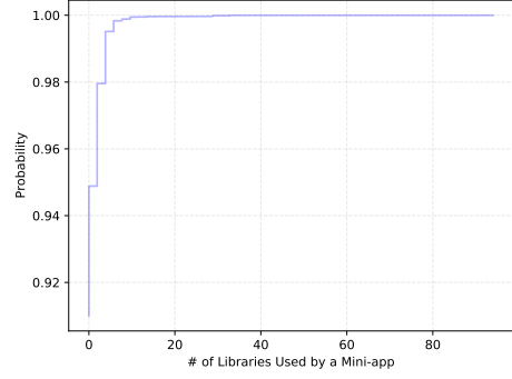
Fig. 22. Distributions of the mini-apps based on the usage of libraries.
