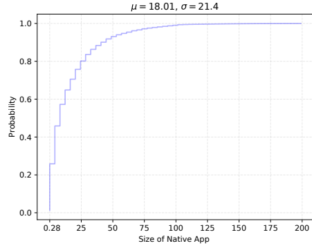
Fig. 10. Size distribution of native apps.
