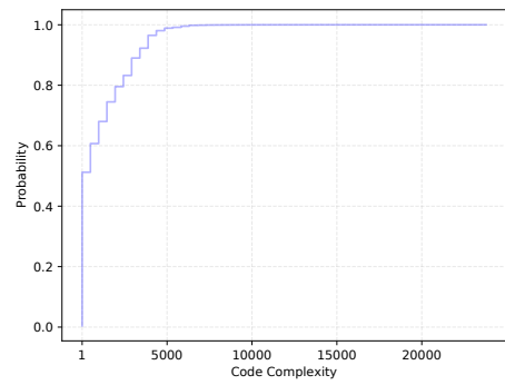
Fig. 14. Distributions of the mini-apps based on the number of code complexity.
