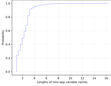
Fig. 21. Distributions of the mini-apps based on the length of variables.
