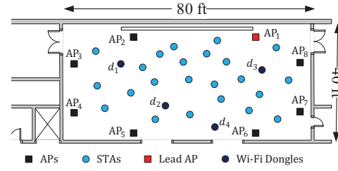
Fig. 12: A conference room for UD-MIMO evaluation.
