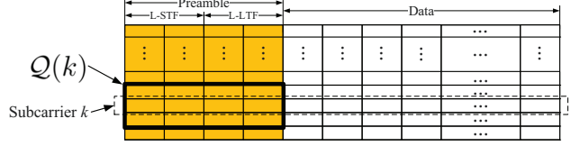
Fig. 9: Illustrating set \mathcal{Q}(k) for filter construction.
