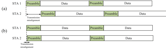
Fig. 10: (a) Transmission misalignment is greater than the time duration of preamble. (b) Transmission misalignment is less than the time duration of CP (guard interval).
