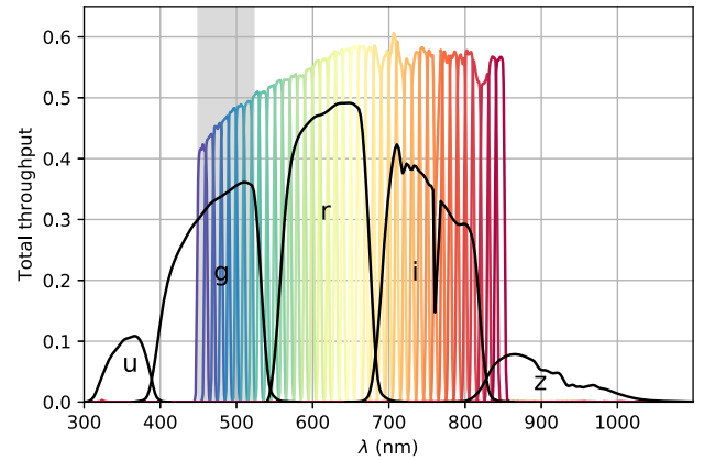
Figure 1. Response function for PAUS filters (coloured) and original SDSS ugriz filters (black). Shaded area represents the wavelength range studied in this work.
