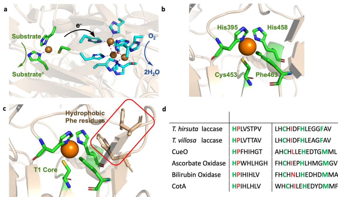
Figure 1. (a) The active site of fungal laccase from Trametes hirsuta (PDB:3fpx) showing the electron transfer from the T1Cu center to the site of O 2 reduction at the trinuclear copper center in MCOs. (b) The T1Cu center of the fungal laccase from T. hirsuta . (c) The hydrophobic Phe residues in the SCS of fungal laccase are shown in tan and the T1Cu center is highlighted in green. (d) Sequence alignment of MCOs showing the PCS in green of the T1Cu center and the analogous sites for hydrogen bonding to the S(Cys) residue shown in red. MCOs have a conserved Pro residue in the analogous azurin Asn47 position indicating one hydrogen bond to the S(Cys) rather than two.
