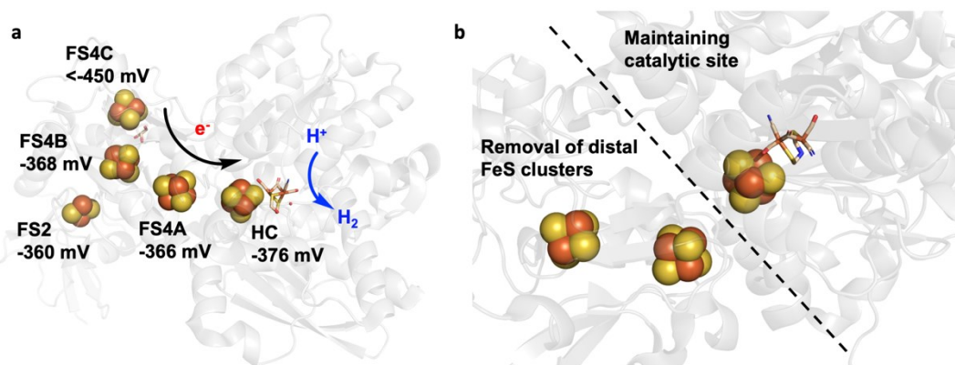
Figure 3. (a) The active site and accessory [FeS] cluster array in CPI [FeFe] hydrogenase (PDB 3C8Y). The reduction potential of each [FeS] cluster was determined and labeled. The proposed electron transfer array from distal [4Fe-4S] cluster to the active site
