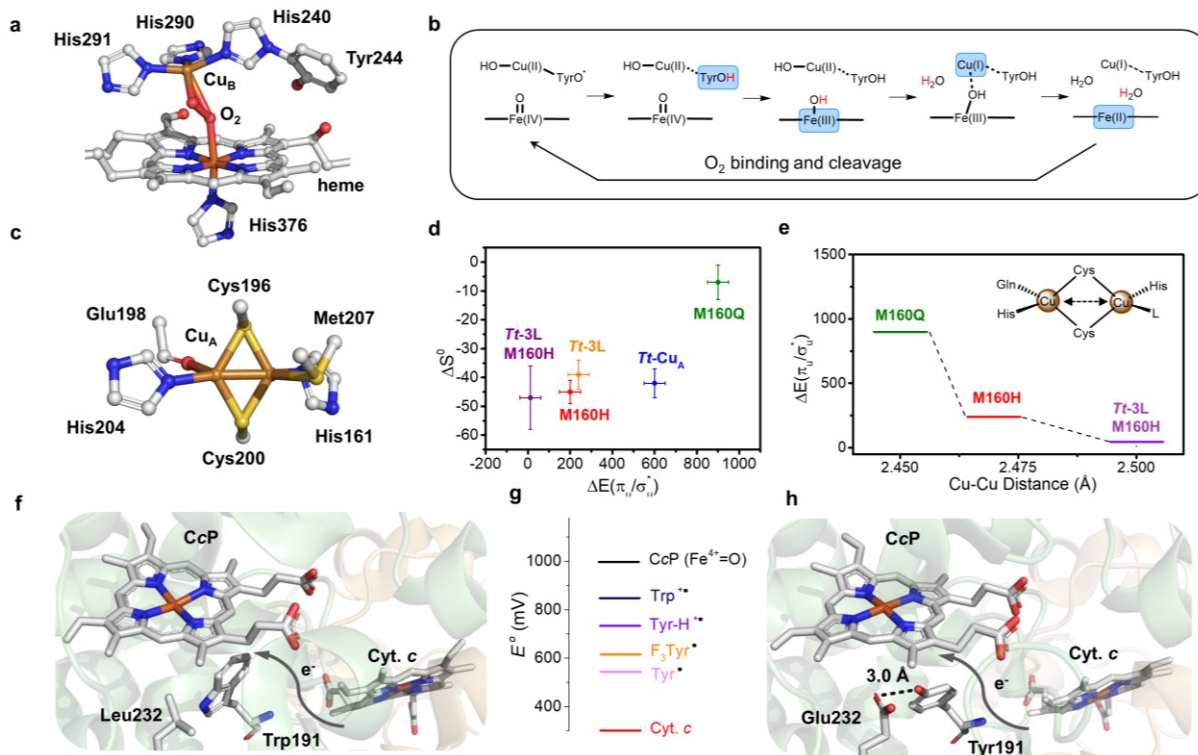
Figure 2. (a) Heme-Cu B site (BNC) of bovine heart HCO (PDB 2OCC) with O 2 bound. (b) Proposed mechanism for HCO which shows the four-electron reduction from fully oxidized BNC to the rest state. Each arrow on the top represents a one-proton-one-electron reduction. The reduced moieties in each step are showed in blue blocks and the coupled protons are labelled in red. (c) Active site structure of Tt -Cu A (PDB 2CUA). (d) Scatter plot of the Cu(II)-Cu(I) entropy change ( \Delta S^0 , y-axis) of Tt -Cu A mutants versus the energy gap between two thermally accessible ground states ( \Delta E_{\sigma_u^*/\pi_u} , x-axis). (e) Change of \Delta E_{\sigma_u^*/\pi_u} (y-axis) with different Cu-Cu distances in Tt -Cu A mutants. (f) Structural representation of wild-type yeast CcP (co-crystallized with Cyt. c, PDB 2PCC). (g) Scheme of reduction potentials of different amino acid residue radicals and iron species. (h) Structural representation of W191Y/L232E CcP (PDB 6P41). The hydrogen bond between Glu232 and Tyr191 is shown as a black dash.
