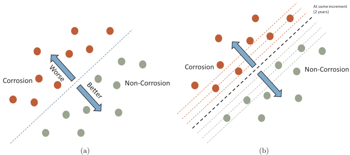
Figure 13. (a) Arbitrary Incremental Corrosion (b) Defined Incremental Corrosion
