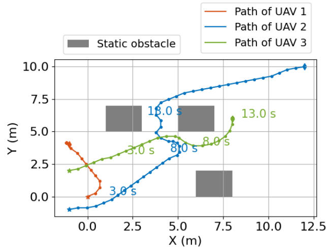
Figure 8: Trajectories of the UAVs operating in a small-scale environment when directly applying the DRL.
