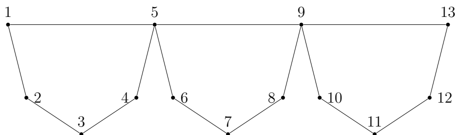
Figure 6: An example of a snake graph C_{5,1}^3 . This snake has a cyclic snake prime labeling.
