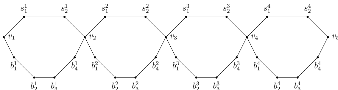
Figure 2: The snake graph C_{8,3}^4 . The spine of the snake, the minimal path of length qm between vertices v_1 and v_5 , can be observed along the top of the figure. The belly of the snake, the path of length (k - q)m between vertices v_1 and v_5 , can be seen along the bottom of the figure.
