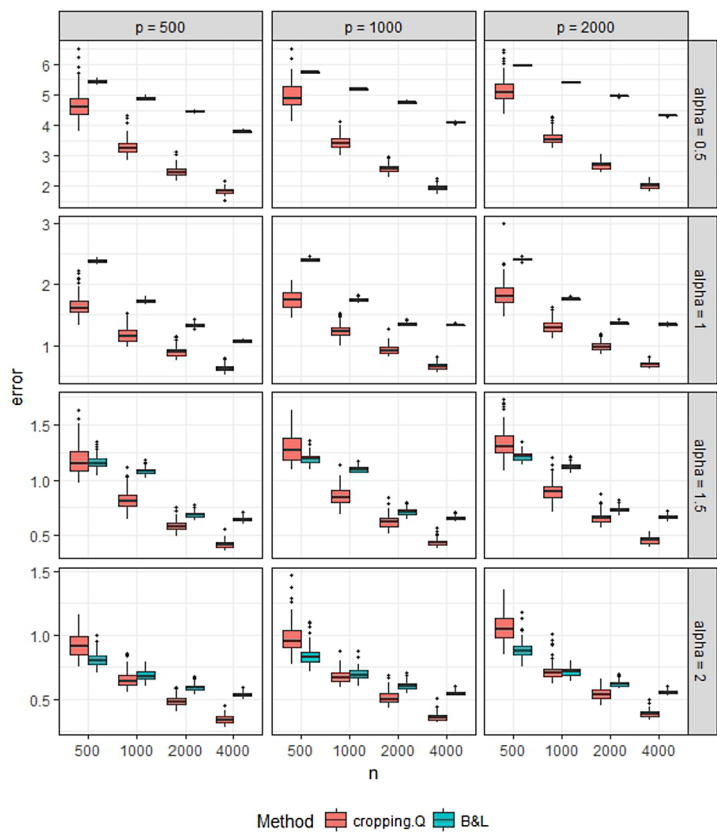
FIG. 2. The boxplot of the errors from the local cropping estimator with the optimal bandwidth in \mathcal{Q}_\alpha(\eta, M) (cropping.Q) and the banding estimator (BL) over 100 replications.
