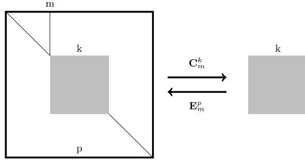
FIG. 1. An illustration of the cropping operator and the expanding operator.
