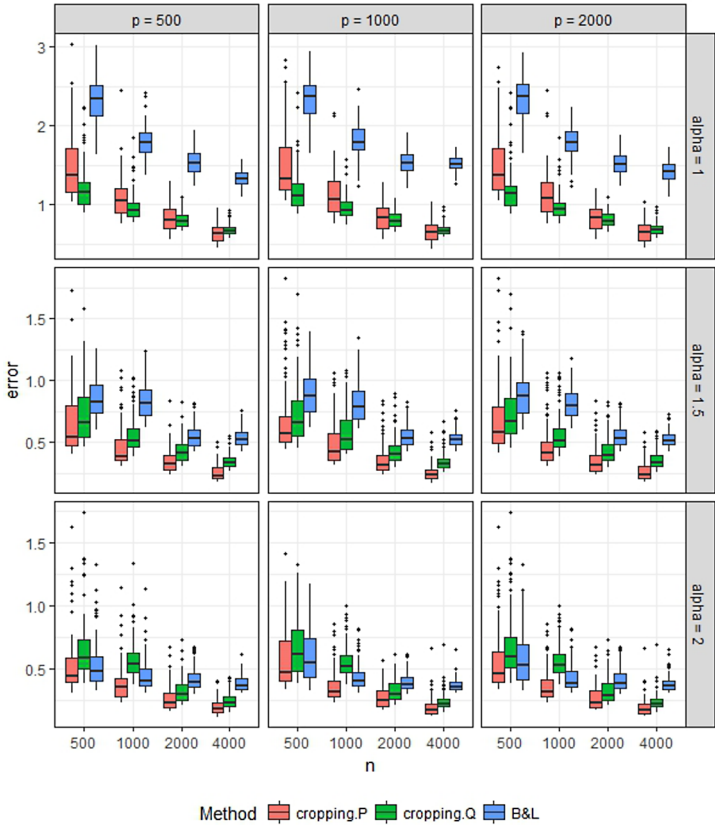
FIG. 3. The boxplot of the errors from the local cropping estimator with the optimal bandwidth in \mathcal{P}_\alpha(\eta, M) (cropping.P), the local cropping estimator with the optimal bandwidth in \mathcal{Q}_\alpha(\eta, M) (cropping.Q) and the banding estimator (BL) over 100 replications.
