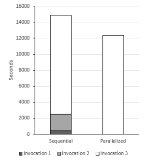
Figure 7: Execution time with Sequential vs. Parallelized library invocations in MetaCompare.
