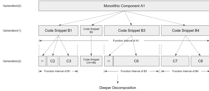
Figure 4: A sample evolution of the decomposition on a monolithic application. Each code snippet is decomposed into a set of multiple smaller functions. If the overall performance of the resulting set is better than the preceding set, then we keep the resulting set, otherwise the original set is preserved.
