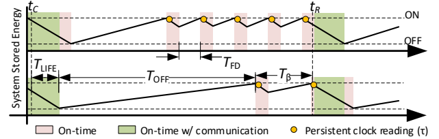
Fig. 5. Clk-LMP. During communication, nodes agree on a rendezvous time t_R , and then use fast-die cycling to try to overlap at this time.
