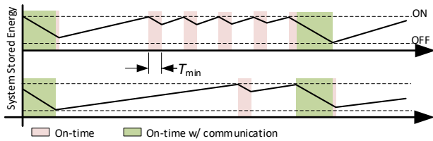
Fig. 4. Fast-LMP. Every time a node revives, it remains on for T_{\min} . Here the two nodes are initially communicating, and happen to overlap later in the figure as well.
