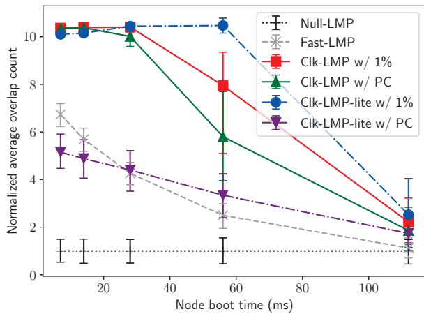
Fig. 13. Normalized average overlap count vs. node bootstrap time.
