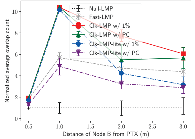
Fig. 11. Normalized average overlap count vs. distance from the PTX. The notation “w/ 1%” means the protocol uses 1% modeled clock error, and “w/ PC” indicates the use of the experimental persistent clock error data.
