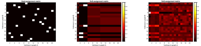
(a) Permutation relating \mathcal{G}_A and \mathcal{G}_B . (b) Optimal solution of our formulation. (c) Optimal solution of prevailing formulation.
