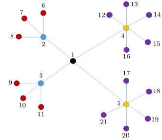
Fig. 1: Invariance classes in a graph \mathcal{G}_A . Swapping a pair of vertices of the same color (together with their descendants, if any) does not affect the topology of the graph. Note that a one-to-one correspondence is incapable of revealing the invariance classes.
