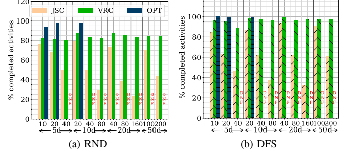
Fig. 4. Fraction (%) of submitted activities scheduled per mission for MNet.
