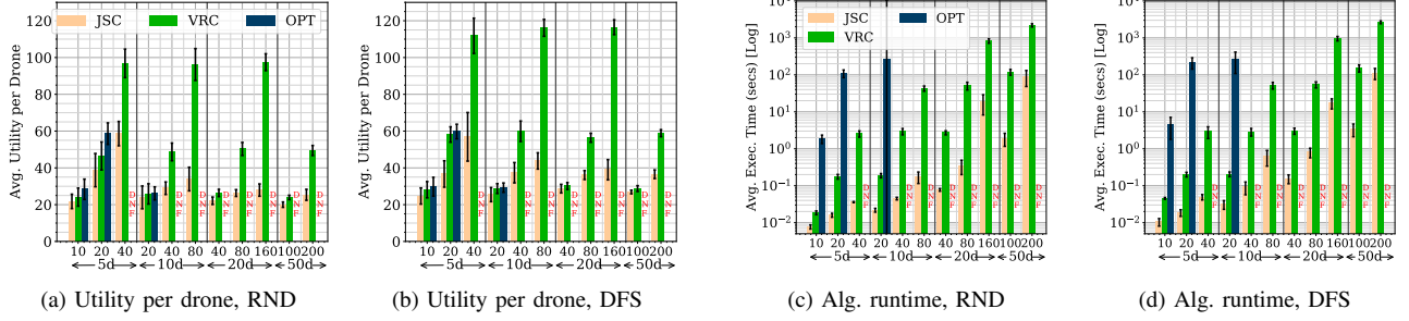
Fig. 2. Expected utility per drone and algorithm runtime of the three MSP algorithms, for the RND and DFS workloads on MNet. On the X axis, the number of drones (outer) and activities per drone (inner) increase. OPT is solved on 16× cores while JSC and VRC run on just 1. DNF indicates OPT did not finish.
