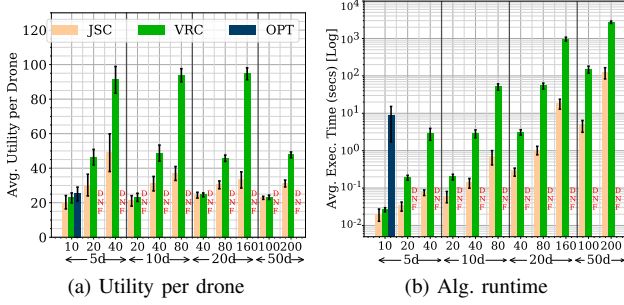
Fig. 3. Expected utility per drone and algorithm runtime for RNet on DFS.
