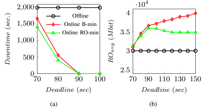
Fig. 12: Overall downtime (a) and (b) average network RO per VM migration with respect to the value of evacuation deadline.
