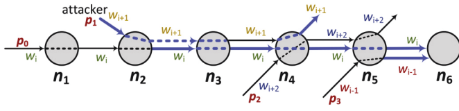
Fig. 16. Propagation of out-of-band jamming attacks in the network (adapted from [161, Fig. 2]).
