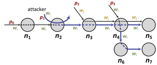
Fig. 15. Propagation of in-band jamming attacks in the network (adapted from [161, Fig. 1]).
