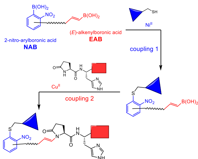
Figure 1. Schematic depiction of the sequential cross-coupling of NAB and EAB boronic acid pairs.
