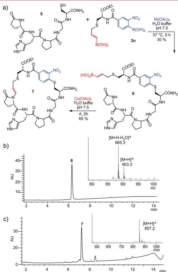
Figure 4. Peptide stapling with sequential boronic acid coupling. (a) Synthetic scheme for the preparation of the peptide staple 7. Conditions: cysteine modification: 5 (0.2 mM), 2n (2 mM), and \text{Ni}(\text{OAc})_2 (1 mM) in NMM buffer (10 mM, pH 7.5), TCEP (1 mM), 37 °C, 5 h; pEH alkenylation: 6 (0.2 mM) and \text{Cu}(\text{OAc})_2 (1 mM) in NMM buffer pH 7.5 for 2 h. (b) LCMS chromatogram of 6 . Insert: mass chromatogram of 6 . (c) LCMS of the crude reaction mixture for the conversion of 6 to 7 . Insert: mass chromatogram of the new peak 7 .
