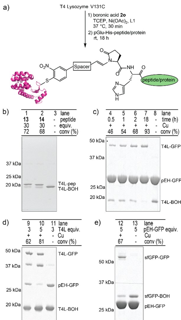
Figure 5. (a) Overview of the conjugation of T4L with pyroglutamate-histidine-tagged structures using diboronic acid 2o . Conditions: (1) T4L (20 \mu M), 2o (200 \mu M), tris(2-carboxyethyl)-phosphine (TCEP) (0.2 mM), Ni(OAc) 2 (0.4 mM), and 6,6'-dimethyl-2,2'-bipyridine (L1) (0.4 mM) in NMM buffer (50 mM, pH 7.5) at 37 °C for 30 min. (2) Boronic-acid-modified T4L (10 \mu M), pGlu-His-peptide/protein (50 \mu M), and Cu(OAc) 2 (0.25 mM) in NMM buffer (50 mM, 150 mM NaCl, pH 7.5) at rt for 18 h. (b–e) Gel images for the conjugation of T4L-boronic acid with (b) pGlu-His peptides and (c) pGlu-His GFP. (d) Conjugation of T4L-boronic acid to pGlu-His-GFP with excess T4L. (e) Conjugation of sfGFP-boronic acid with pGlu-His-GFP. Conversion was measured by gel densitometry (ImageJ) relative to the starting material and was uncalibrated.
