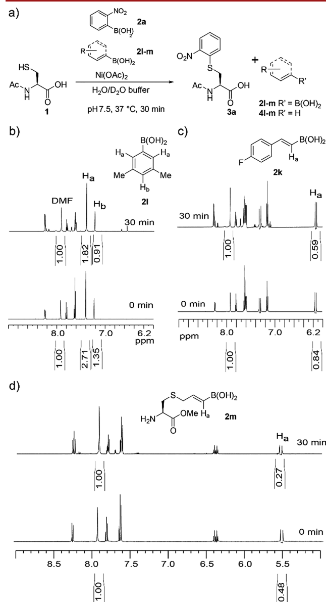
Figure 3. (a) Stability of aryl- and alkenyl-boronic acid reagents in the nickel(II)-mediated reaction. (b,c) NMR monitoring of the stability of “bystander” boronic acids 2l and 2m in an NAB-type Ni 2+ coupling with boronic acid 2a .
