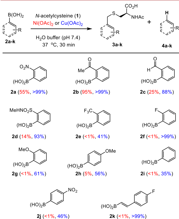
Figure 2. Conversion of boronic acid reagents 2a–k in the presence of Ni 2+ and Cu 2+ salts. The total conversion to products 3 and 4 is shown for Ni 2+ (red) and Cu 2+ (blue). Conditions: boronic acid (2 mM), N -acetylcysteine (0.2 mM), and M(OAc) 2 (1 mM) in aqueous N -methylmorpholine (NMM) buffer (10 mM).
