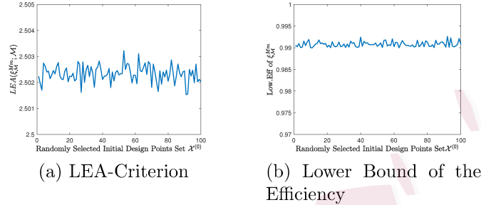
Figure 4: Performance of Algorithm 1 for 100 Randomly Generated \mathcal{X}^{(0)}
