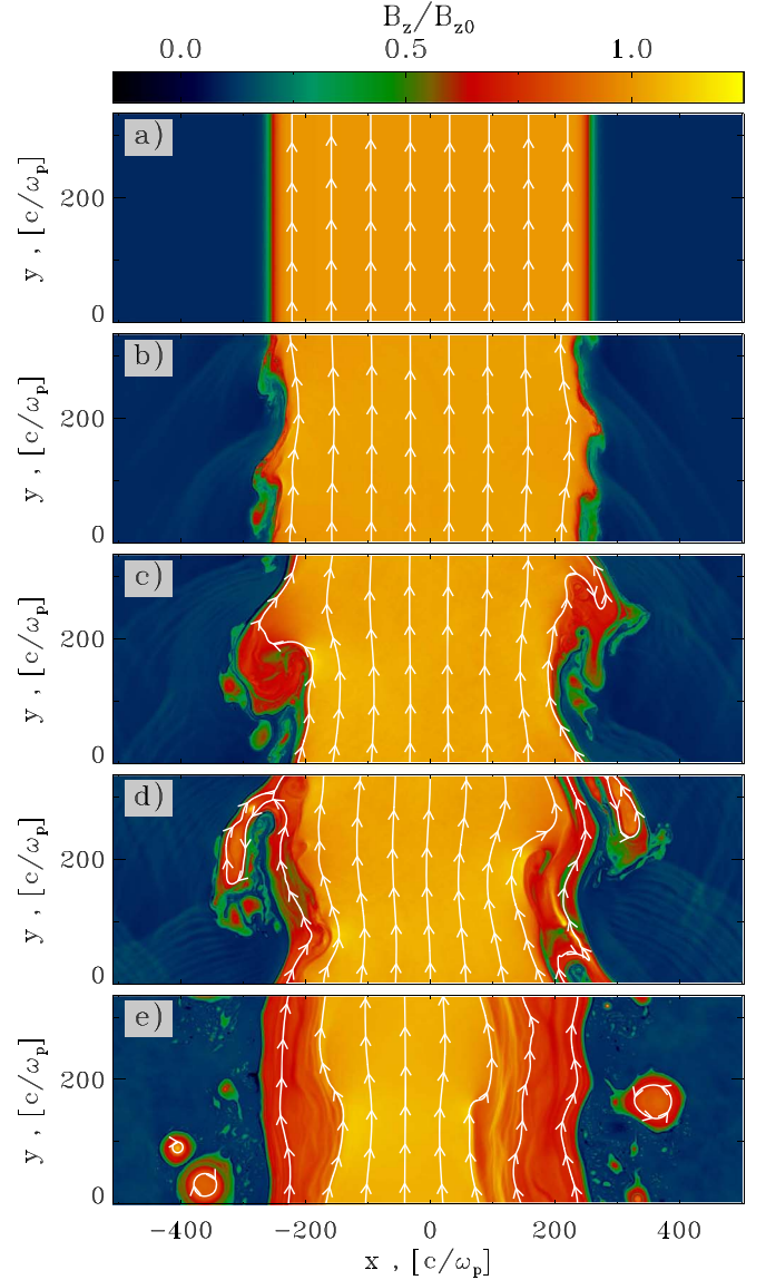
Figure 1. 2D evolution of the out-of-plane field B_z (color)—in units of the initial jet field B_{z0} \equiv B_{j,z} —at (a) \omega_p t = 80 , (b) \omega_p t = 3262 , (c) \omega_p t = 4216 , (d) \omega_p t = 5171 , and (e) \omega_p t = 12569 , with in-plane field lines overlaid. The jet is initially at |x| \lesssim 250 c/\omega_p , surrounded by the wind.
