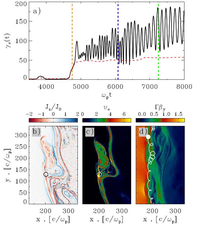
Figure 4. Trajectory of a representative high-energy electron. Panel (a): time evolution of Lorentz factor (solid black line) and parallel work W_{||} = -e \int_0^t E_{||} v_{||} dt' / m_e c^2 (dashed red line), where E_{||} = \mathbf{E} \cdot \hat{\mathbf{b}} and v_{||} = \mathbf{v} \cdot \hat{\mathbf{b}} (here, \mathbf{E} is the electric field, \mathbf{v} the electron velocity, and \hat{\mathbf{b}} = \mathbf{B}/B the magnetic field unit vector). Panels (b) and (c): 2D structure of the out-of-plane current J_z (in units of J_0 = en_0 c ) and of the mean internal energy per electron v_e (in units of m_e c^2 ), at the time \omega_p t = 4750 of particle injection (vertical dashed orange line in (a)). The electron position is indicated by the circle. Panel (d): 2D structure of the bulk four-velocity along y , in units of c , at \omega_p t \approx 7250 (vertical dashed green line in (a)). The electron position at this time is indicated by the filled circle, and we also plot its trajectory from \omega_p t = 6080 (blue dashed line in (a)) to \omega_p t = 7250 (green dashed line in (a)).
