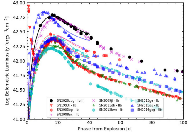
Figure 5. Pseudo-bolometric light curves of SN 1993J, SN 2003bg, SN 2008ax, SN 2009jf, SN 2011dh, iPTF13bvn, SN 2013ge, SN 2015ap, SN 2016gkg, and SN 2020cpg, covering a period of 100 d from their estimated explosion date. The Arnett-like model fit to the pseudo-bolometric light curves, detailed in Section 3.2, are shown as lines and were fitted out to \sim 40 d before they started to strongly diverge from the pseudo-bolometric light curves. The velocities used to break the degeneracy for each SN, along with the predicted physical parameters, are given in Table 4.
