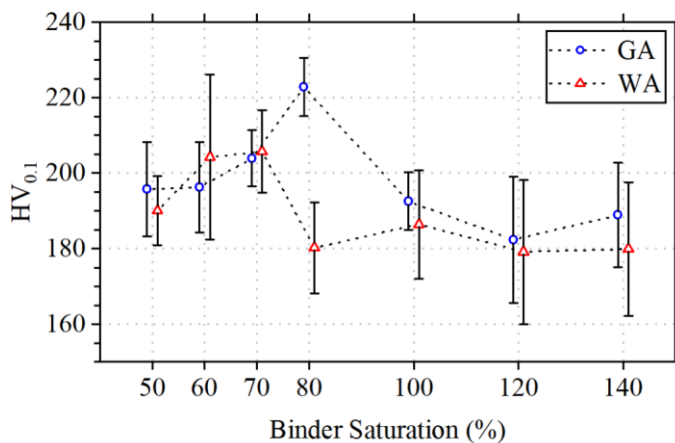
Figure 9. Vickers microhardness values of the sintered WA and GA Inconel 625 samples printed at different binder saturation levels.
