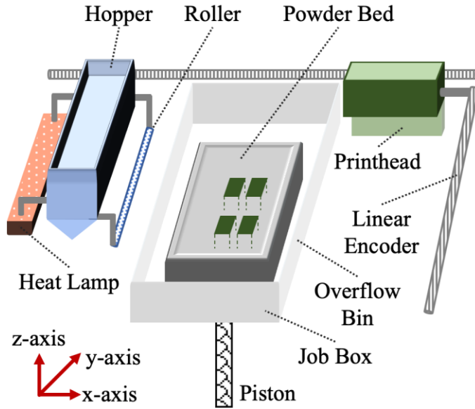
Figure 1. Schematic illustration of the ExOne Innovent binder jet 3D printer with the printing directions specified by the red arrows (not drawn to scale).
