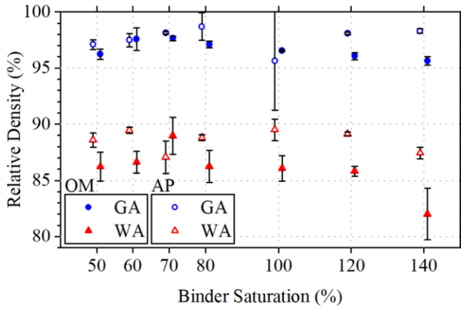
Figure 7. Relative density measured from image analysis of optical micrographs (solid data points) and Archimedes method (hollow data points) of the sintered Inconel 625 samples printed with different binder saturation levels. Data points of binder saturation are staggered for better comprehensibility.
