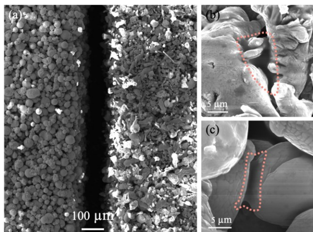
Supplemental figure 14. SEM micrographs of cured (a) green parts with the left being a GA sample and right being a WA sample, and pendular bonds are clearly shown in cured (b) WA and (c) GA Inconel 625 samples
