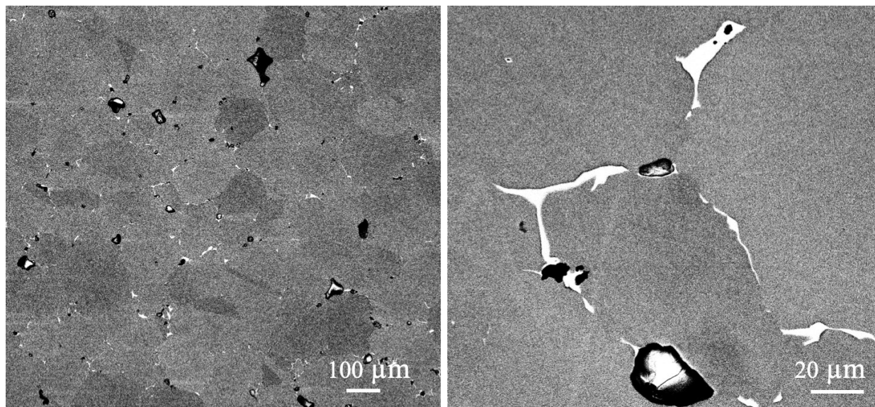
Supplemental figure 13. Exemplary BSE mode SEM micrographs of the sintered BJP GA IN625 alloy with 140% binder saturation. The extent of elemental segregation was much lower in GA samples compared with WA cases.
