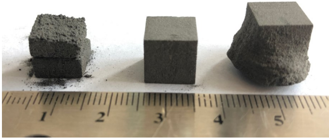
Figure 2. Photograph of the common BJP AM in-process defects from binder saturation: from left to right insufficient saturation, adequate saturation, and excessive saturation. The digital model for all three samples is designed to be a 10 \times 10 \times 10 mm cube.
