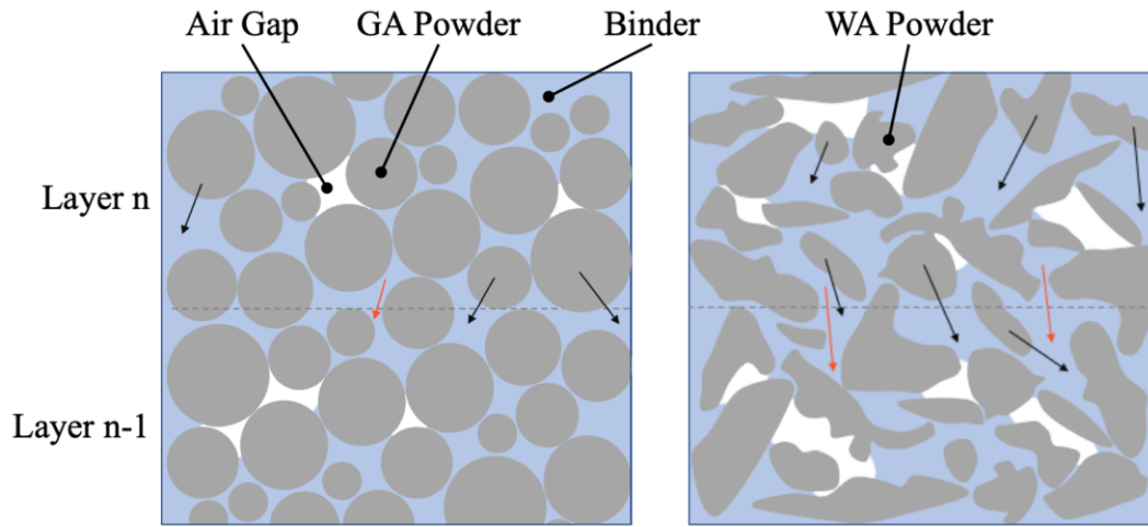
Figure 10. Schematic diagram showing the mechanisms of the binder bleeding phenomenon in the powder bed of (a) spherical GA powder and (b) irregular WA powder. Layer n is the current layer, and layer n-1 is the one printed before layer n. Red arrows indicate the excessive binder migrates in the previously printed layers and lateral unsaturated areas; black arrows indicate the binder dragging the powder down which promotes the densification of the n-1 layer.
