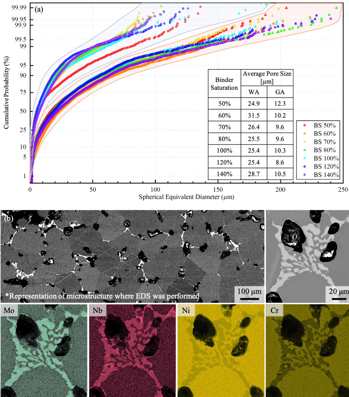
Figure 8. Porosity and elemental analysis of the sintered IN625 structure (a) cumulative probability plot of the pore size distribution from various sintered IN625 structure acquired from optical micrographs and ImageJ analysis. (b) BSE mode SEM micrograph and EDS elemental mappings of the cross-sections of sintered BJP WA IN625 alloy with 140% binder saturation.
