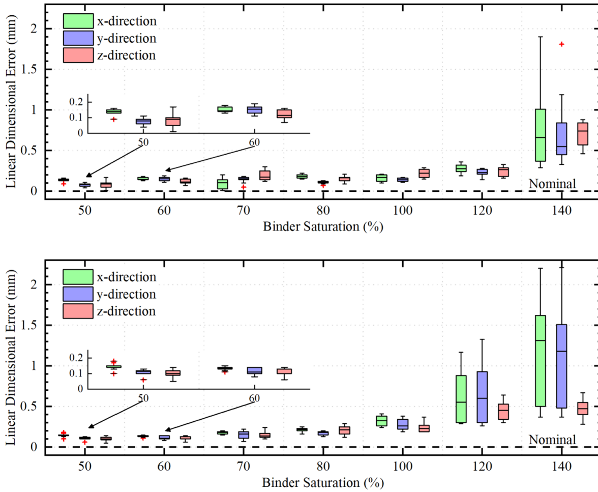
Figure 6. Linear dimensional error of green parts fabricated from the (top) GA and (bottom) WA Inconel 625 alloy powders with various binder saturation levels.
