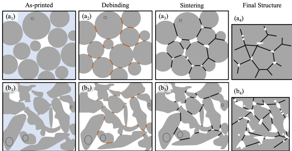
Figure 11. Schematic illustration showing the general process in two dimensions for a binder jet printing system of (a) spherical powder and (b) irregular powder: (a 1 ,b 1 ) as-printed powders, (a 2 ,b 2 ) debound powders which are bonded by pendular bonds, (a 3 ,b 3 ) powders as they begin to adopt the shape of a polyhedron in three dimensions and to enclose the pore channels at the grain boundaries during sintering, and (a 4 ,b 4 ) enclosed pores at the corners where polyhedrons meet present in the final sintered structure.
