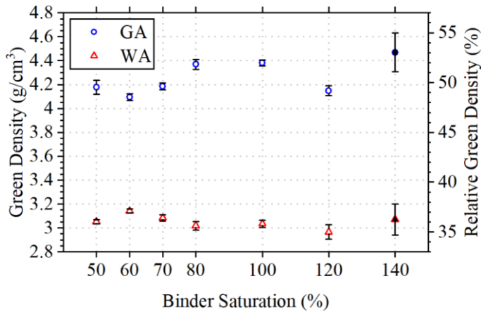
Figure 5. Green part density of Inconel 625 samples of GA and WA Inconel 625 printed with different binder saturation levels. Note that green density values for 140% binder saturation, which are marked as black data points, are not accurate due to the inaccurate measurement of volume caused by extensive binder bleeding.
