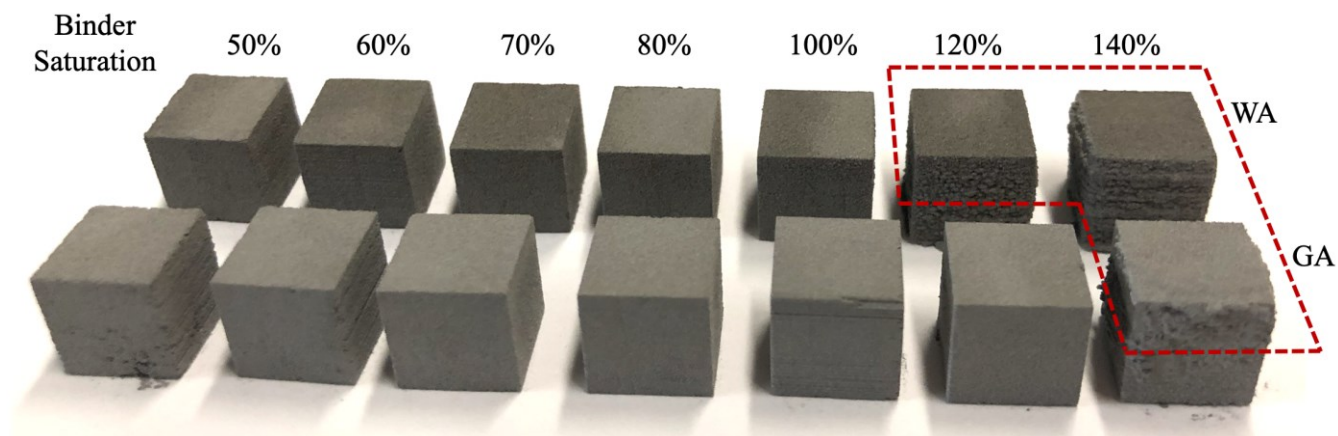
Supplemental figure 12. Image of green parts from WA and GA Inconel 625 alloy printed with different binder saturation levels.
