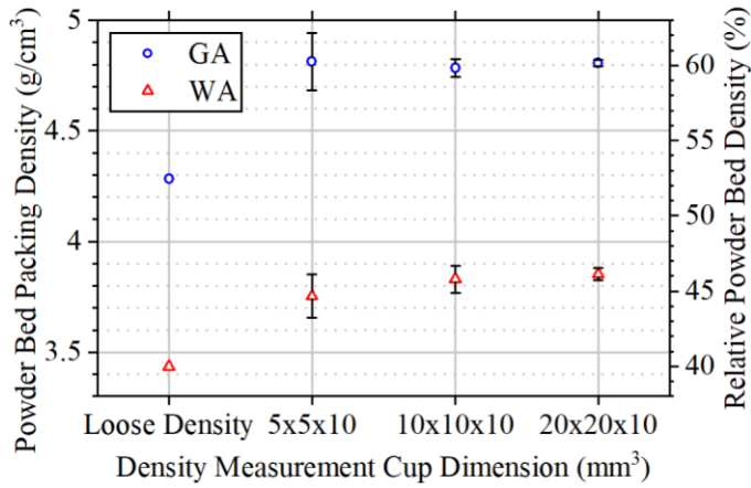
Figure 4. Powder bed packing density of the GA and WA IN625 alloy as measured in the density measurement cups.
