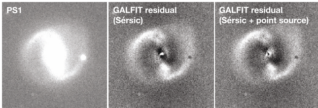
Figure 7. Left: PanSTARRS g -band image of the host galaxy. North is up, and east is towards the left of the image. We fit a Sérsic function for the overall surface brightness profile using GALFIT, but make no attempt to model the spiral arms. The model also includes a point source for the nearby star to the west, and optionally a central point source for the galactic nucleus. Middle: subtraction residuals without a central point source. Right: subtraction residuals when including a central point source. We find visibly smoother residuals in this case.
