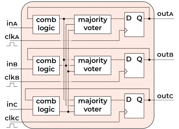
Fig. 8. Full module triplication is used for the I 2 C peripheral. All combinational logic within the module is triplicated, which is used by three majority voters to form the inputs to triplicated registers. Feedback from the output of the registers enables autocorrection and protects against accumulating errors due to single event upsets over time.
