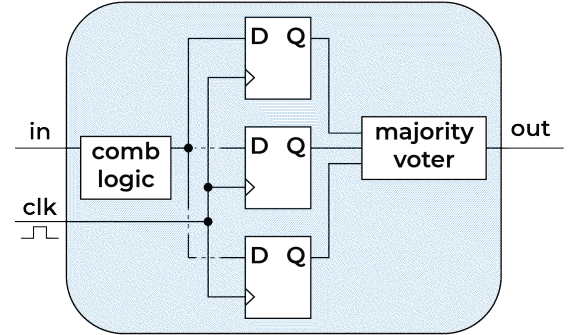
Fig. 7. Triple modular redundancy scheme used for the encoder and converter. Each register is triplicated and a majority voter determines the output.
