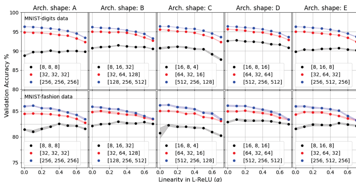
Figure 2. The maximum validation accuracy as a function of the linearity factor ( \alpha ) for models with five network architecture shapes (Arch. shapes A–E) and three network widths (see Table 1). Models were trained on 20,000 MNIST-digits images ( upper panel ) and 20,000 MNIST-fashion images ( lower panel ). For all the models used in this test, the number of nodes used in each hidden layer is shown within the square brackets in each sub-figure in the order of number of nodes used in first, second and third hidden layers, respectively.
