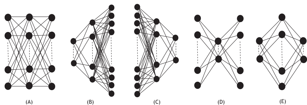
Figure 1. Illustrations in (A–E) are the five model architecture shapes used in the analysis. For each architecture shape, number of nodes per hidden layer was varied according to Table 1, in order to change the model complexity.
