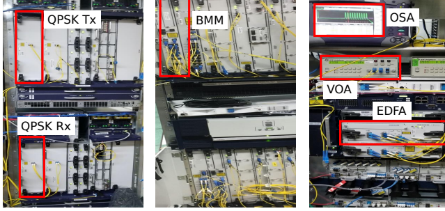
Figure 5: 100 Gbps QPSK transponders (left), band multiplexer (center), optical spectrum analyzer, variable optical attenuator, and erbium doped fiber amplifiers (right).
