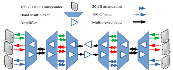
Figure 4: Configuration used in our lab-based experiments: six optical transponders, each of which generate 100 Gbps of Optical Data Unit (ODU) traffic over seven amplifiers.
