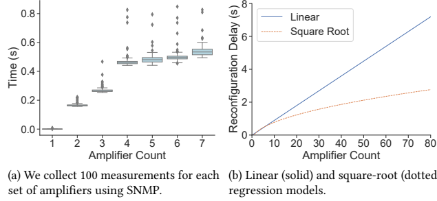
Figure 3: Gain retrieval time for a path of seven amplifiers (3a), and projected reconfiguration time for longer paths (3b).
