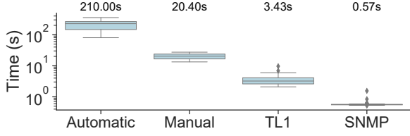
Figure 2: Reconfiguration delays for various modes (mean value shown above).
