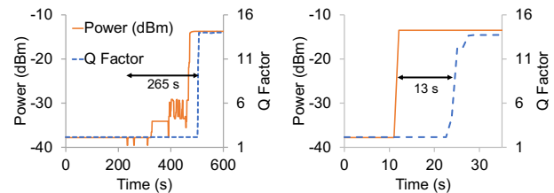
(a) Automatic mode: add-time is 4 min and 25 s. Hence, today's WANs are not OTP-ready. (b) Manual mode: add-time is 13 s—over 19× faster than automatic mode (Figure 1a).
