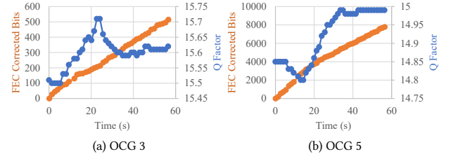
Figure 6: QoT measurements for witness waves while adding/dropping OCG1. During the add/drop, Q factor for the witness waves is relatively constant—varying by \pm 0.1 . Errors accumulate at a linear rate as expected in a live transport network; 100% are corrected with FEC while running traffic over OCGs 3 and 5.
