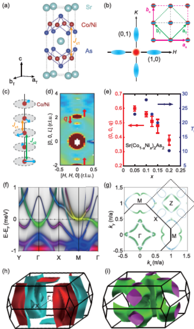
FIG. 1. (a) Crystal structure of \text{Sr}(\text{Co}_{1-x}\text{Ni}_x)_2\text{As}_2 . (b) Schematics of spin fluctuations in reciprocal space and the Co lattice in real space. Red (blue) areas represent FM (AF) spin fluctuations. (c) Helical magnetic structure in the x = 0.1 compound. (d) Neutron diffraction intensity in the [H, H, L] plane. The red arrows indicate the helical wave vector. (e) Magnetic wave vectors and 3D transition temperatures in \text{Sr}(\text{Co}_{1-x}\text{Ni}_x)_2\text{As}_2 . (f) Electronic band structures and the Fermi surfaces for k_z = 0 in x = 0.1 . Green (red) color represents the d_{x^2-y^2} ( d_{z^2} ) orbital and blue is the contribution from the t_{2g} ( d_{xz}, d_{yz}, d_{xy} ) orbitals. Yellow is the mixture of the red ( d_{z^2} ) and green ( d_{x^2-y^2} ). (h), (i) Calculated 3D Fermi surfaces of the x = 0.1 compound.
