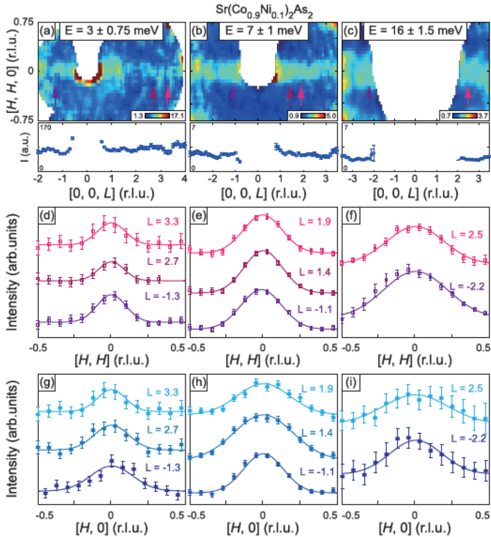
FIG. 4. (a)–(c) Constant energy slices of spin fluctuations of \text{Sr}(\text{Co}_{0.9}\text{Ni}_{0.1})_2\text{As}_2 within the [H, H, L] plane at E = 3 \pm 0.75 , 7 \pm 1 , and 16 \pm 1.5 meV, respectively. The corresponding 1D cuts along the [0, 0, L] direction are shown in the bottom panel. (d)–(f) 1D cuts of spin fluctuations along the [H, H] direction at different L and energies. (g)–(i) Corresponding 1D cuts along the [H, 0] direction. The solid lines are Gaussian fits to the cuts.
