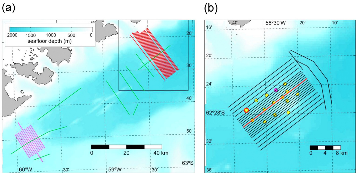
Fig. 6. (a) MCS profiles carried out over Orca volcano (red), Humpback volcano (purple), and in the Bransfield rift (green). (b) Shooting profiles carried out over the seismic instruments surrounding Orca volcano (black), for tomography and refraction studies. The shots of the profile marked in red, recorded at the OBS encircled in red, are displayed in Fig. 15. The area zoomed in (b) is marked by a black box in (a). (For interpretation of the references to color in this figure legend, the reader is referred to the Web version of this article.)
