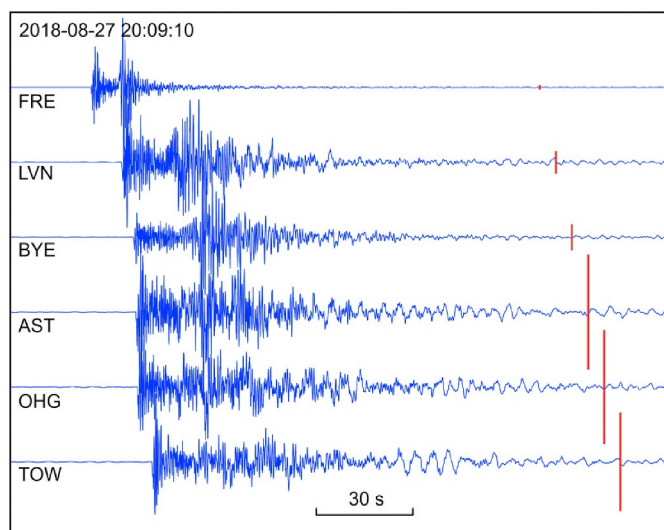
Fig. 7. Seismograms (vertical component) of a M5.6 tectonic earthquake recorded by land seismometers in the Bransfield Strait area on August 27, 2018. Data are normalized to their maxima; the red bars on the right side indicate the relative seismogram amplitudes. The start time of the records is indicated at the top left. (For interpretation of the references to color in this figure legend, the reader is referred to the Web version of this article.)
