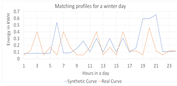
Figure 6: Best real curve match for a sample synthetic curve for winter using DTW and radius 3.
