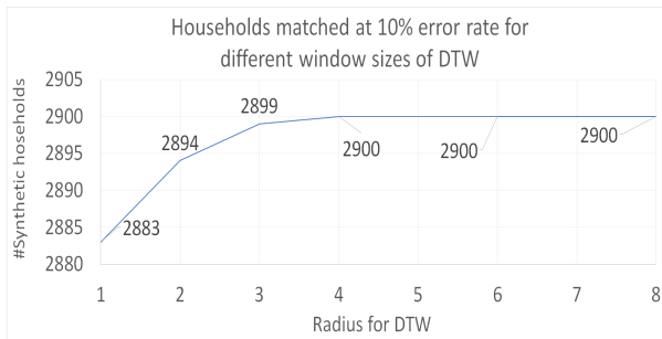
Figure 8: An elbow plot representing the number of synthetic households in Rappahannock county that fall within 10% error rate for different window sizes (radius or w ) of DTW matching process. We choose w=3 .
