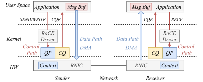
Figure 1: RDMA Transmission Mechanism
