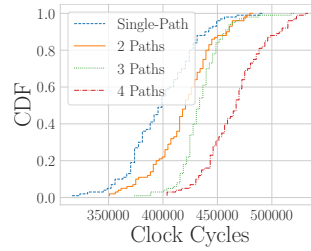
Figure 13: CPU Overhead
