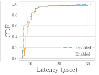
Figure 14: Aggressiveness
