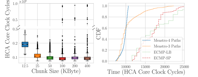
Figure 9: Chunk Size
