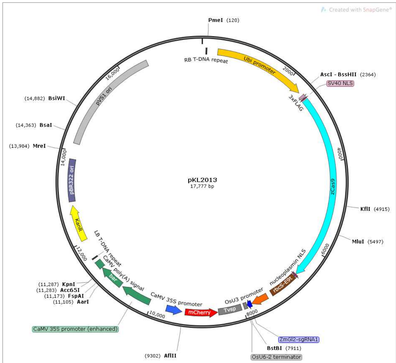
Figure S1. Map of pKL2013.
